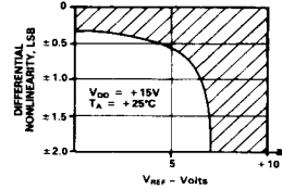
Figure 4. Differential Nonlinearity vs. Reference Voltage (Shaded Area Shows Range of Values of DNL That Typically Occur for K and J Grades)
