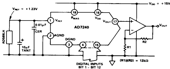
Figure 12. AD7240 in Single Supply Voltage Switching Mode
