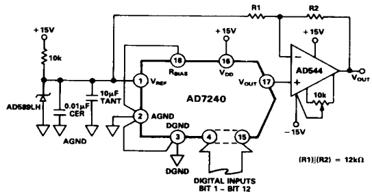
Figure 14. AD7240 in Offset-Binary Voltage-Switching Mode
