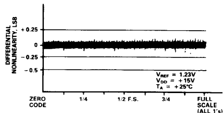
Figure 6. Differential Nonlinearity vs. Digital Code
