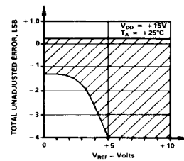
Figure 2. Total Error vs. Reference Voltage (Shaded Area Shows Range of Values of Total Unadjusted Error That Typically Occurs for AD7240JN)
