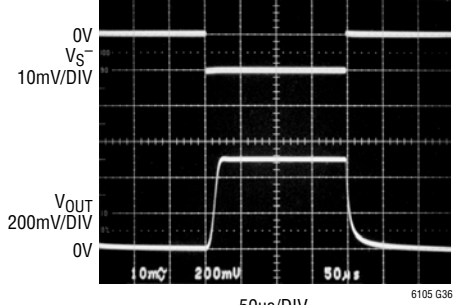
Step Response V_{SENSE} = 0V \text{ to } 10mV, V_S^+ = 0V
