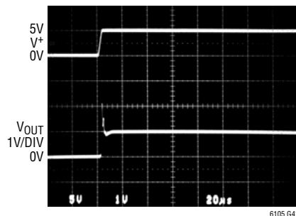
Power Supply Start-Up Response
