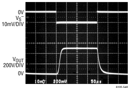
Step Response V_{SENSE} = 0V \text{ to } 10mV, C_L = 1000pF, V_S^+ = 0V
