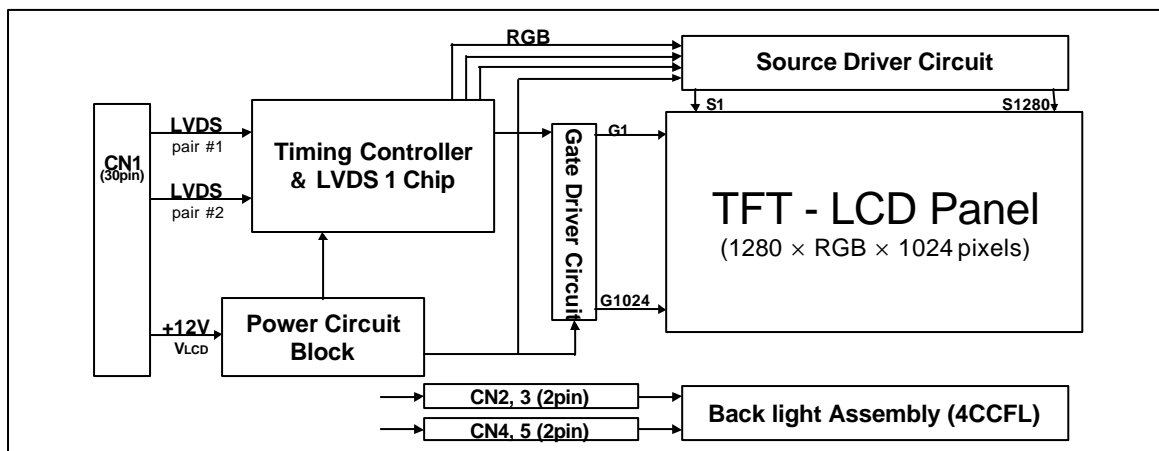
Figure 1. Block diagram
