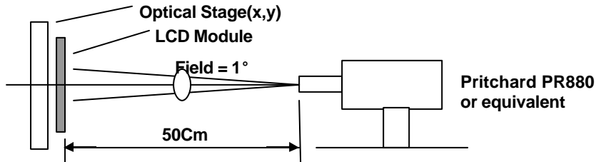
[Figure 9] Optical characteristic measurement equipment and method
