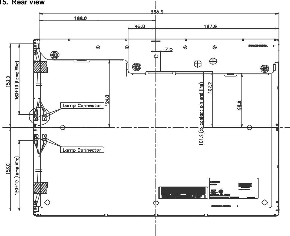
Figure 15. Rear view
