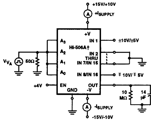
FIGURE 5B. TEST CIRCUIT
