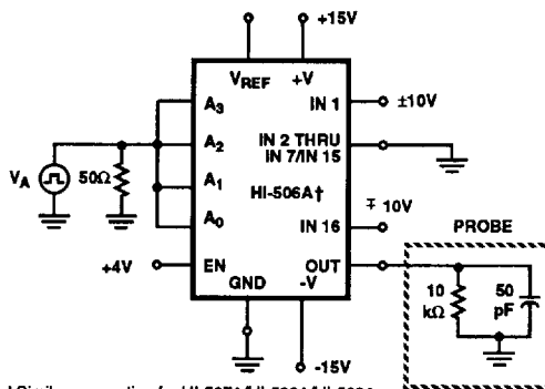
FIGURE 6B. TEST CIRCUIT
