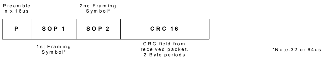
Figure 6-2. Example ACK Packet Format
