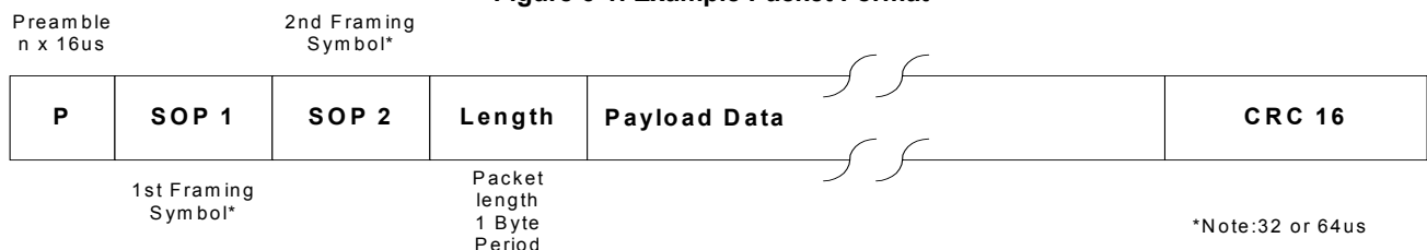
Figure 6-1. Example Packet Format
