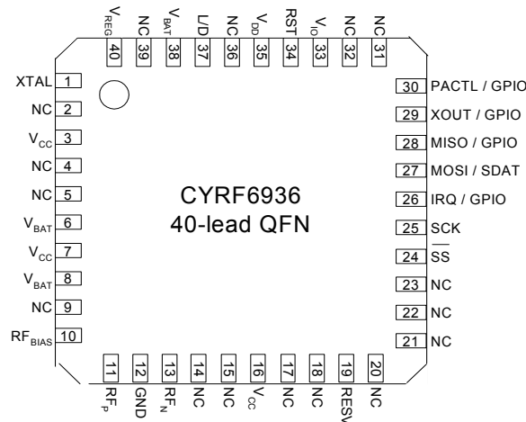
Figure 5-1. CYRF6936, 40 QFN – Top Vie CYRF6936 Top View*
