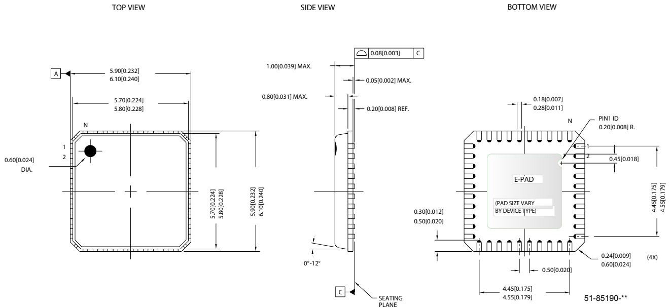
Figure 18-1. 40-pin Lead-Free QFN 6x6 mm LY40
