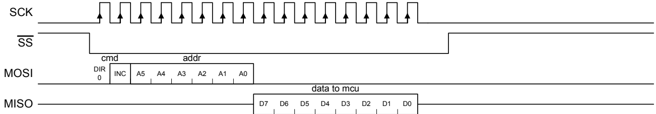
Figure 7-2. SPI Single Read Sequence
