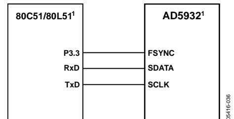
1 ADDITIONAL PINS OMITTED FOR CLARITY. Figure 36. 80C51/80L51 to AD5932 Interface
