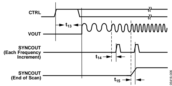
Figure 6. SYNCOUT Timing
