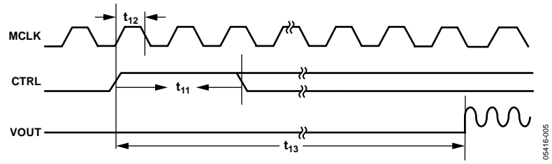
Figure 5. CTRL Timing
