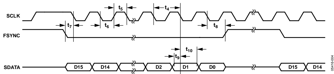
Figure 4. Serial Timing
