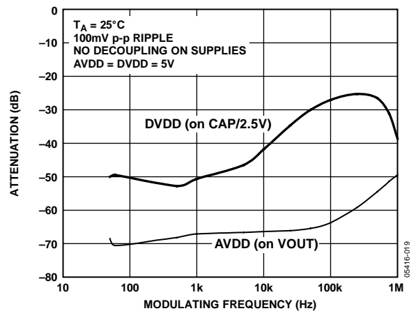
Figure 19. PSRR
