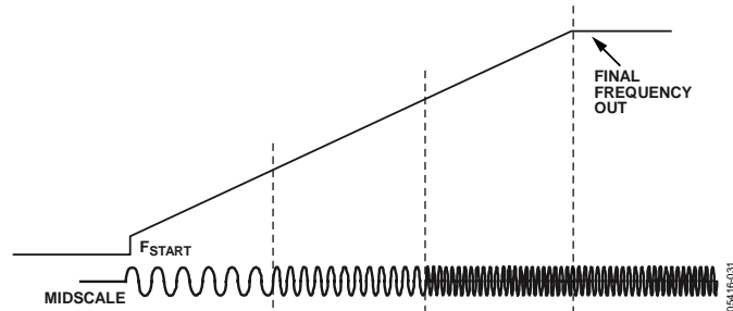
Figure 31. Frequency Scan
