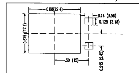
Min. Recommended Footprint Dimensions in inches and mm)
