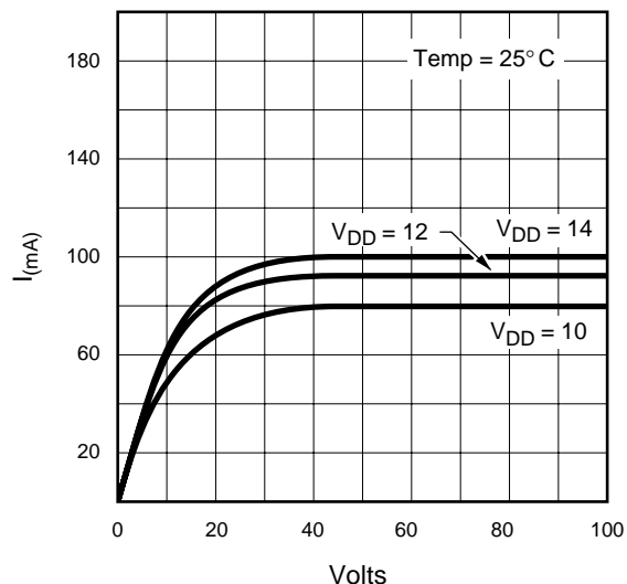
Output N-Channel Characteristics through FET
