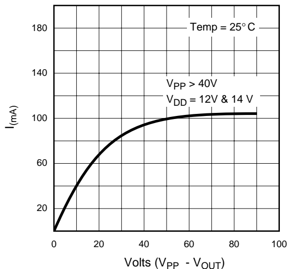
Output P-Channel Characteristics through FET
