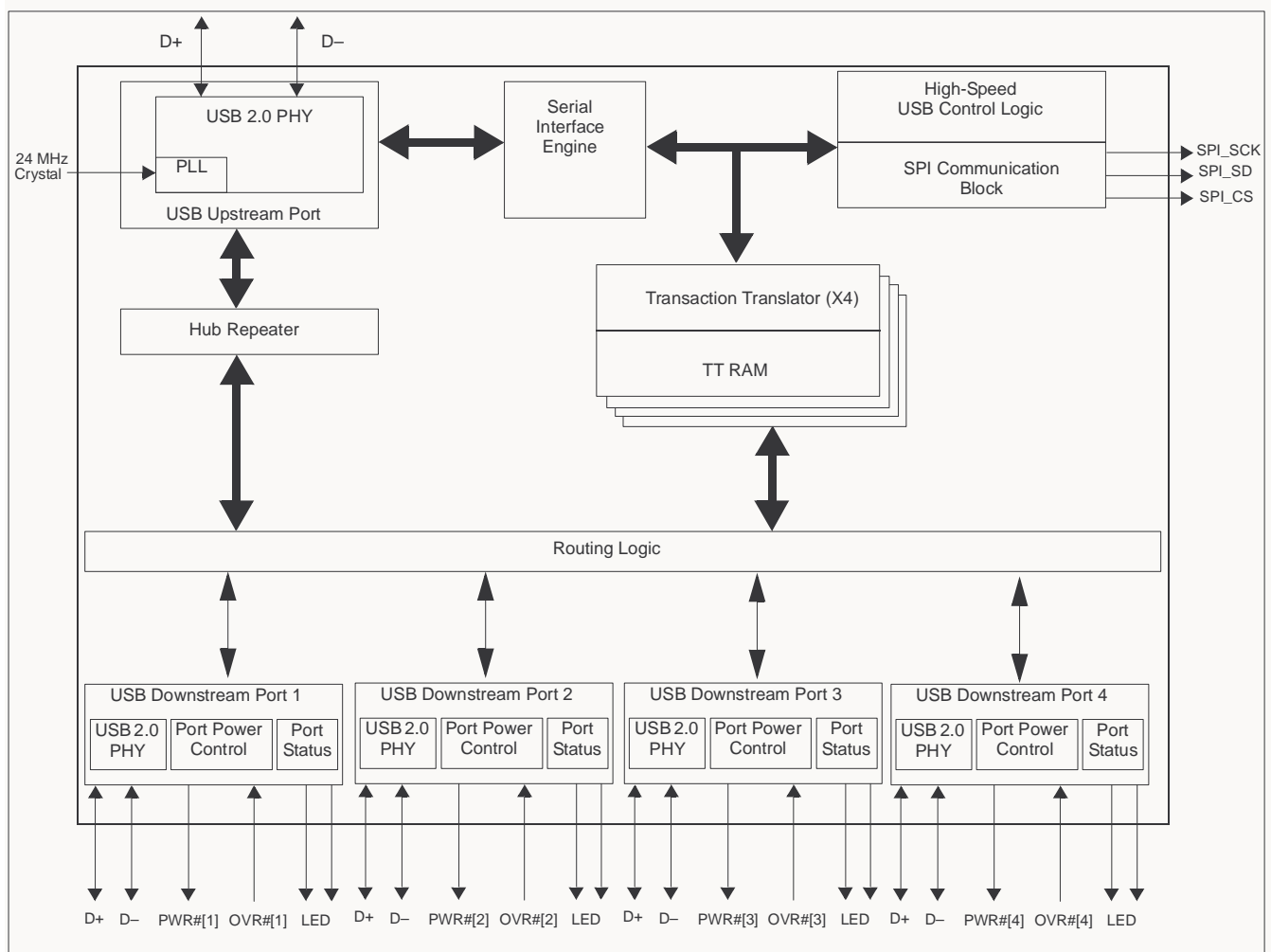
Figure 1-1. Block Diagram
