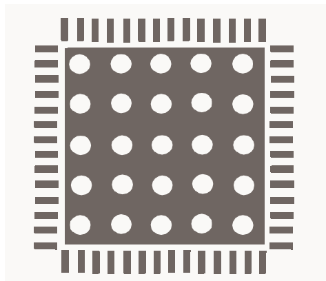
Figure 16-2a. Plot of the Solder Mask (White Area)
