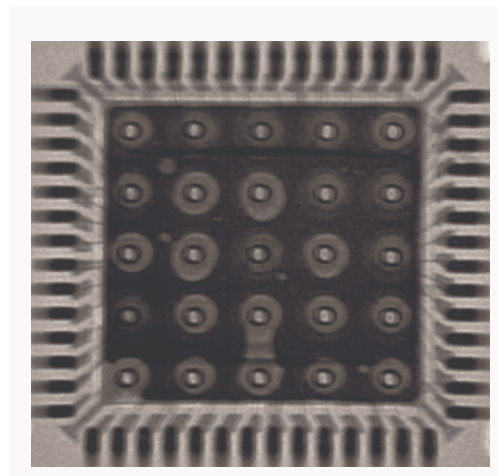
Figure 16-2b. X-Ray Image of the Assembly
