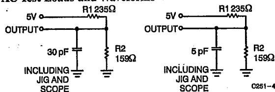
(b) High Z Load
