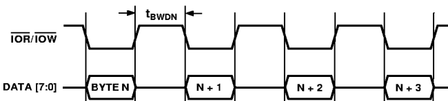
Figure 5. Codec Transfers
