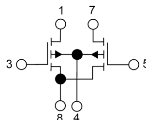
Device Schematic
