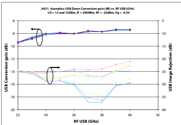
IF=200 MHz
