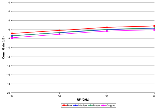
XM1002, LSB Conversion Gain (6566 devices)
