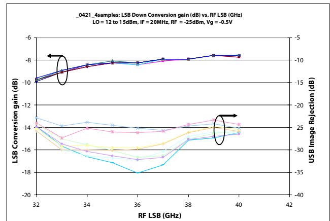
IF=20 MHz
