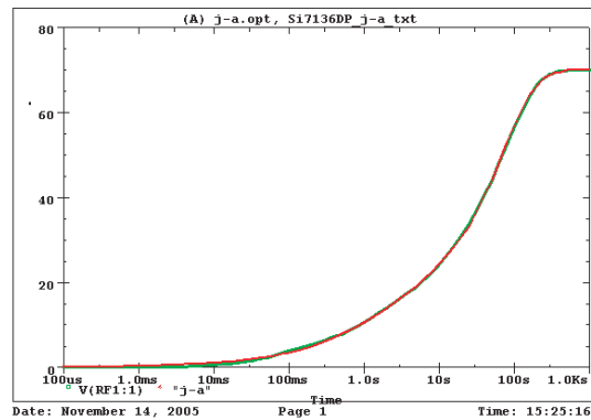
Si7136DP Filter j-a Temperature: 27.0
