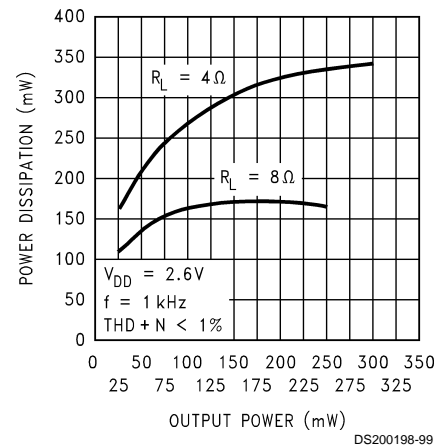
Power Dissipation vs Output Power, 2.6V, 8 \Omega and 4 \Omega
