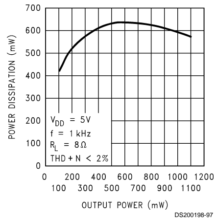
Power Dissipation vs Output Power, 5V, 8 \Omega
