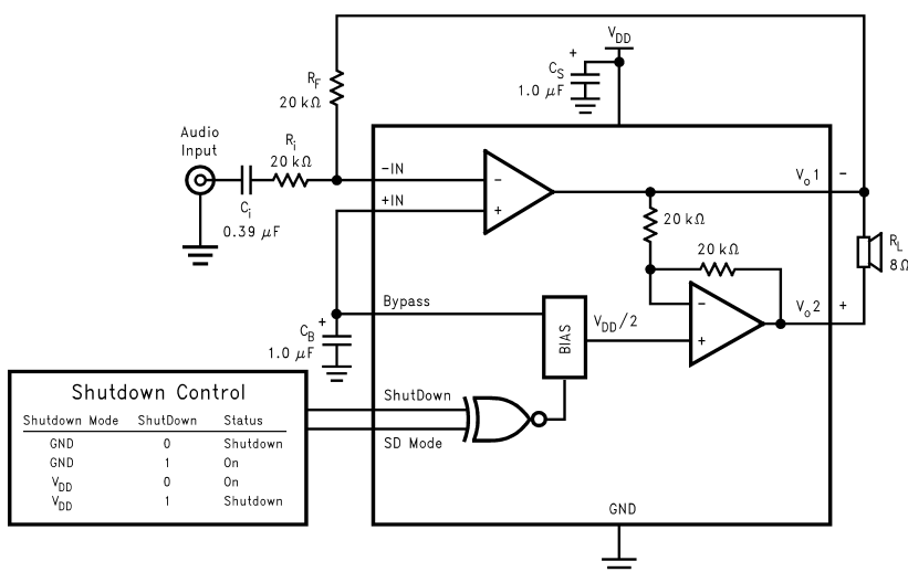
FIGURE 1. Typical Audio Amplifier Application Circuit
