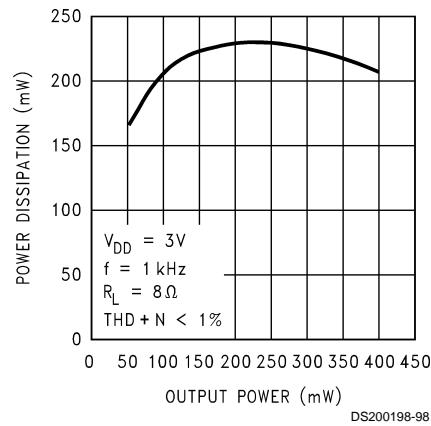
Power Dissipation vs Output Power, 3V, 8 \Omega
