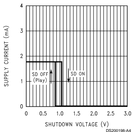
Shutdown Hysteresis Voltage 2.6V, SD Mode = V_{DD} (High)
