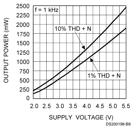
Output Power vs Supply Voltage, 4 \Omega
