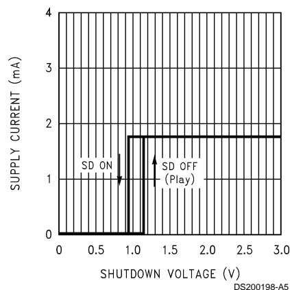
Shutdown Hysteresis Voltage 2.6V, SD Mode = GND (Low)
