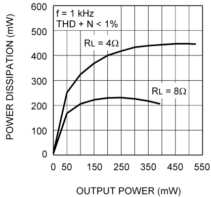
Power Dissipation vs Output Power, V_{DD} = 3V
