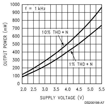
Output Power vs Supply Voltage, 16 \Omega
