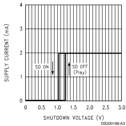
Shutdown Hysteresis Voltage 3V, SD Mode = GND (Low)
