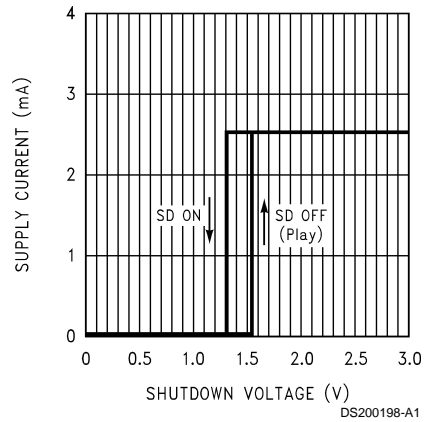
Shutdown Hysteresis Voltage 5V, SD Mode = GND (Low)
