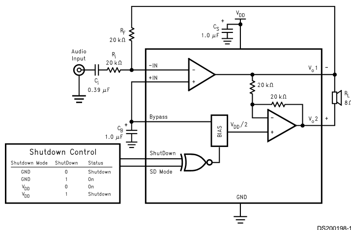
FIGURE 1. Typical Audio Amplifier Application Circuit
