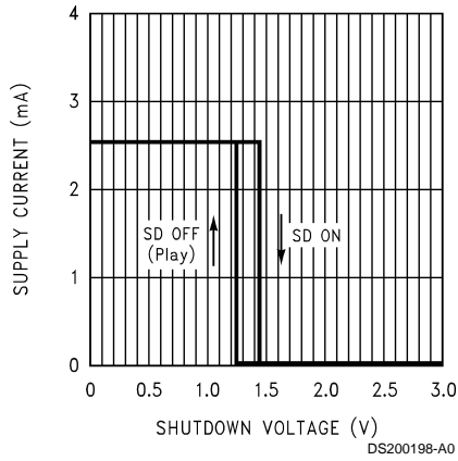
Shutdown Hysteresis Voltage 5V, SD Mode = V_{DD} (High)
