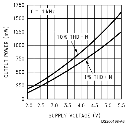
Output Power vs Supply Voltage, 8 \Omega
