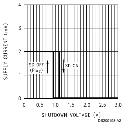
Shutdown Hysteresis Voltage 3V, SD Mode = V_{DD} (High)
