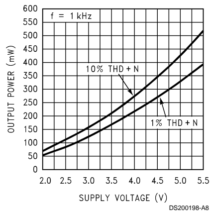
Output Power vs Supply Voltage, 32 \Omega
