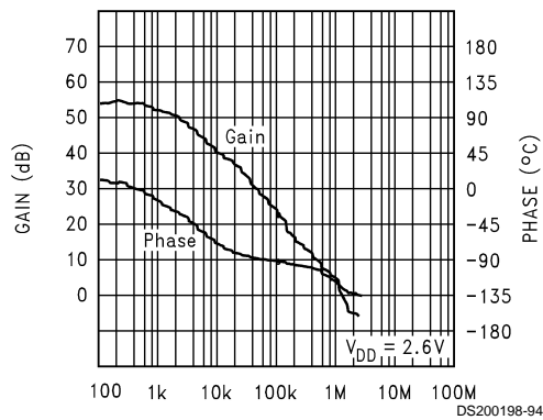
Open Loop Frequency Response, 2.6V
