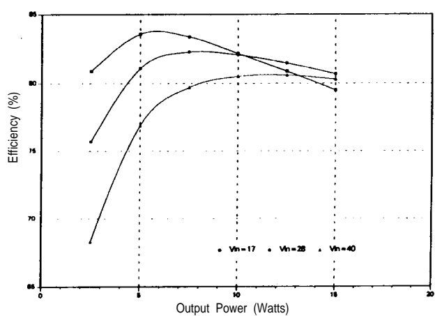
AHE2812S EFFICIENCY
