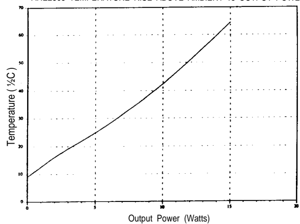
AHE2805 TEMPERATURE RISE ABOVE AMBIENT vs OUTPUT POWER
