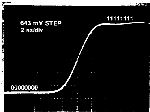
Figure 4. Full Scale Step Rise Time.
