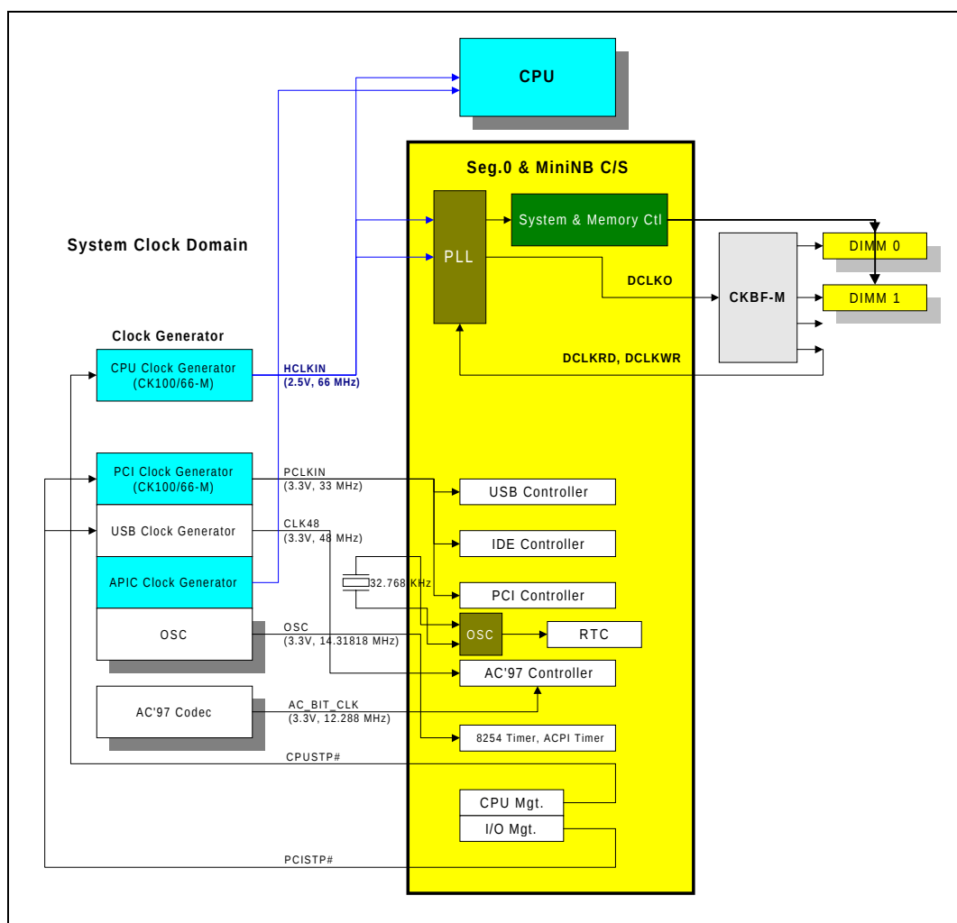
Figure 27. System Clocking
