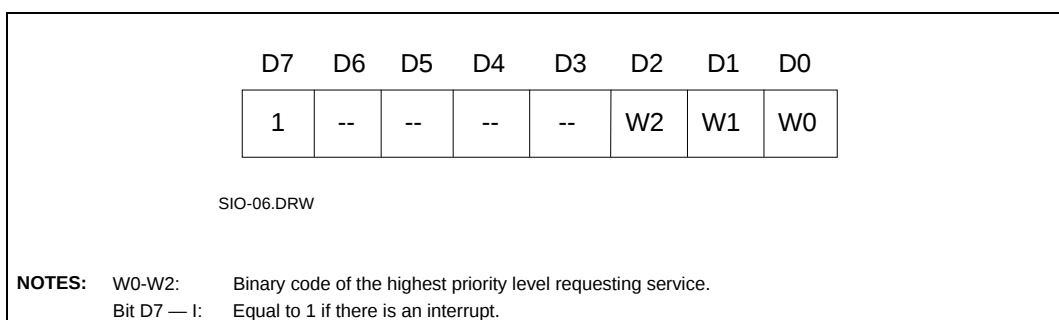
Figure 19. Polled Mode
