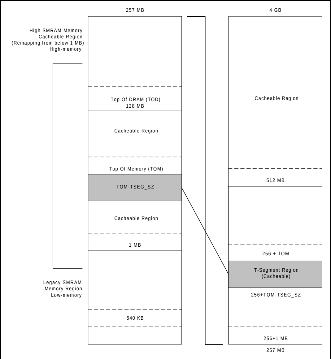
Figure 7. SMRAM Mapping
