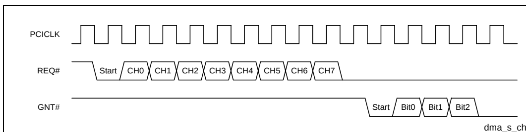
Figure 15. DMA Serial Channel Passing Protocol
