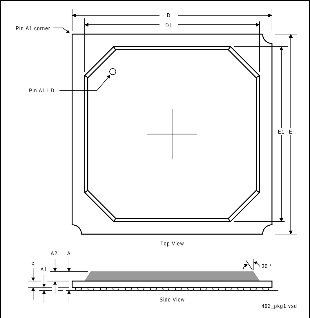
Figure 30. 440MX BGA Package Dimensions (Top and Side View)
