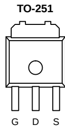
Top View Order Number: SUY50N03-10CP
