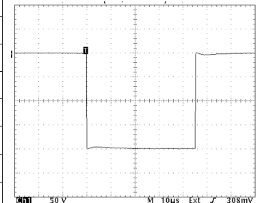
Typical Output Waveform, 200V (10µs/Div horizontal scale, 50V/Div vertical scale)
