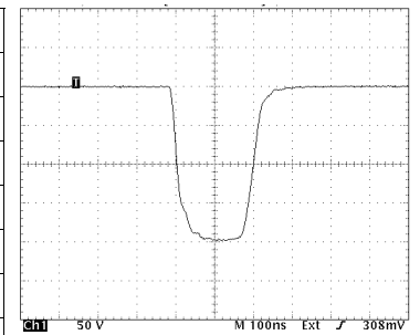
200ns Minimum Pulse Width, 200V Output (100ns/Div horizontal scale, 50V/Div vertical scale)
