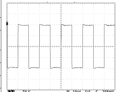
50KHz, 50% Duty Cycle, 200V Output (8Ω Load, 10µs/Div horizontal scale, 50V/Div vertical scale)
