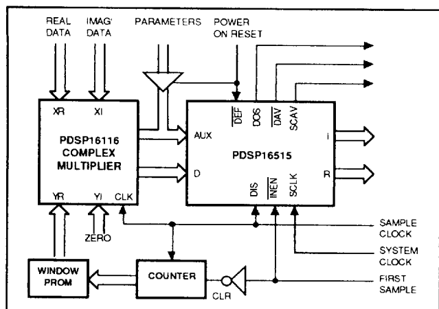
Fig. 11 External Window Generator
