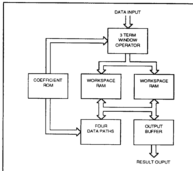
Fig. 1. Block Diagram
