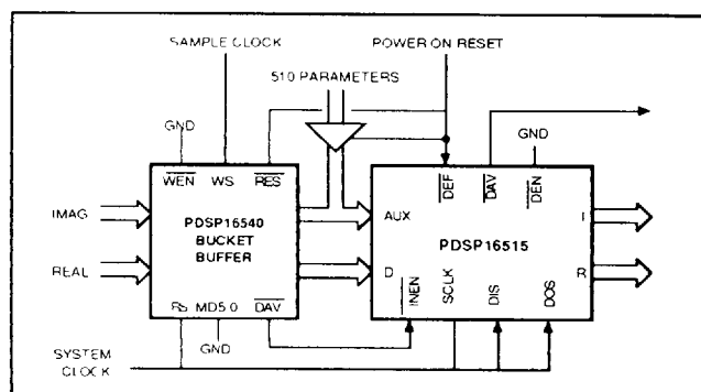
Fig 6 1024 Point Transforms with I/P Buffer
