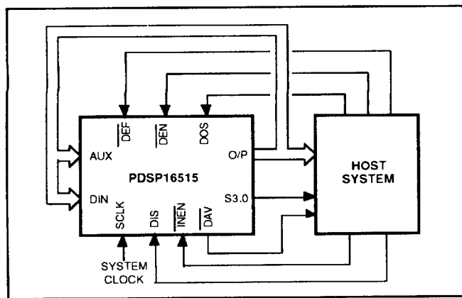
Fig. 7. Host Controlled System
