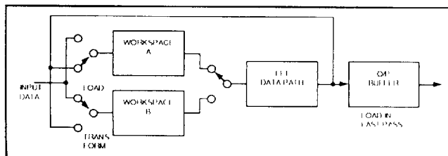
Fig 4 RAM Organization with 256 Data Points
