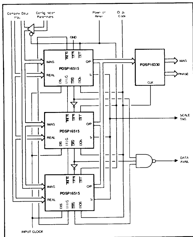
Figure 9 Multiple Device Configuration
