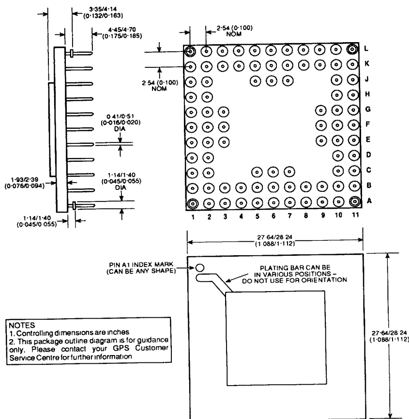
84-PIN GRID ARRAY PACKAGE - AC84
