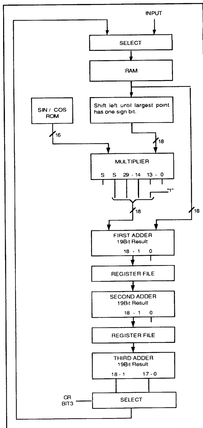
Fig. 3 One of Four Data Paths
