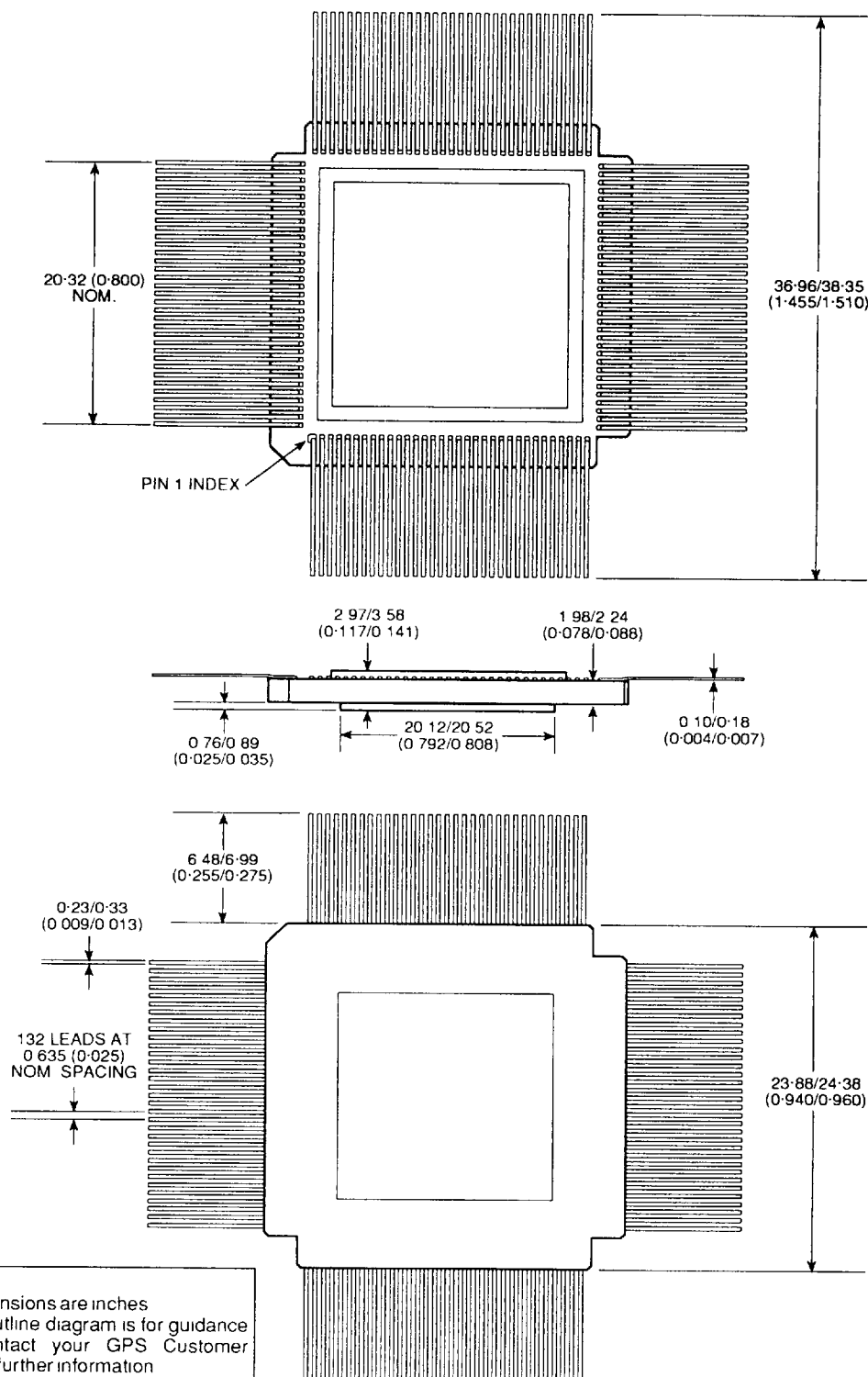
132-PIN POWER CERAMIC QFP - GC132
