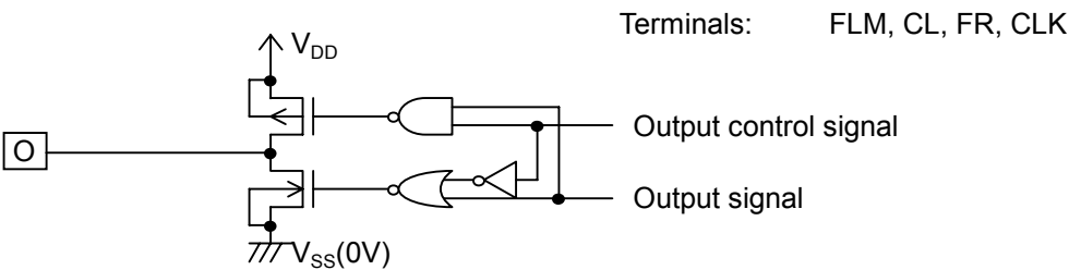
(b) Output circuit
