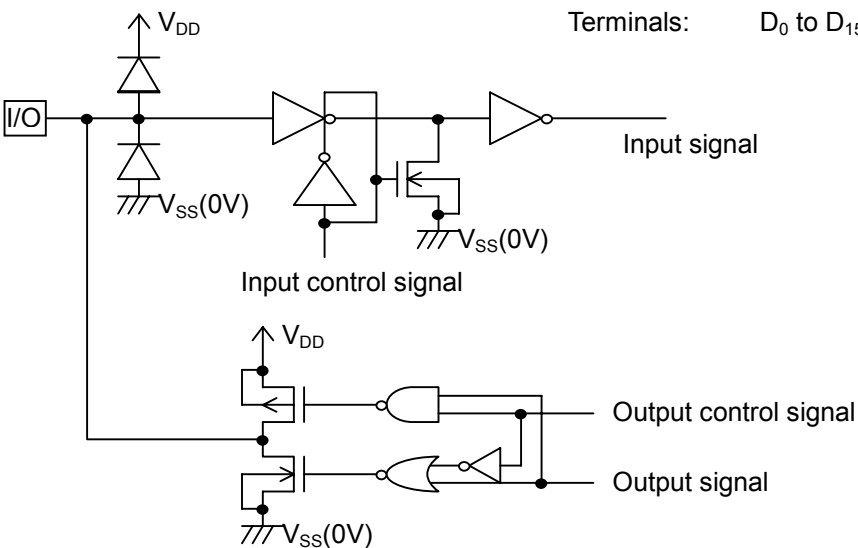
(c) Input/Output circuit
