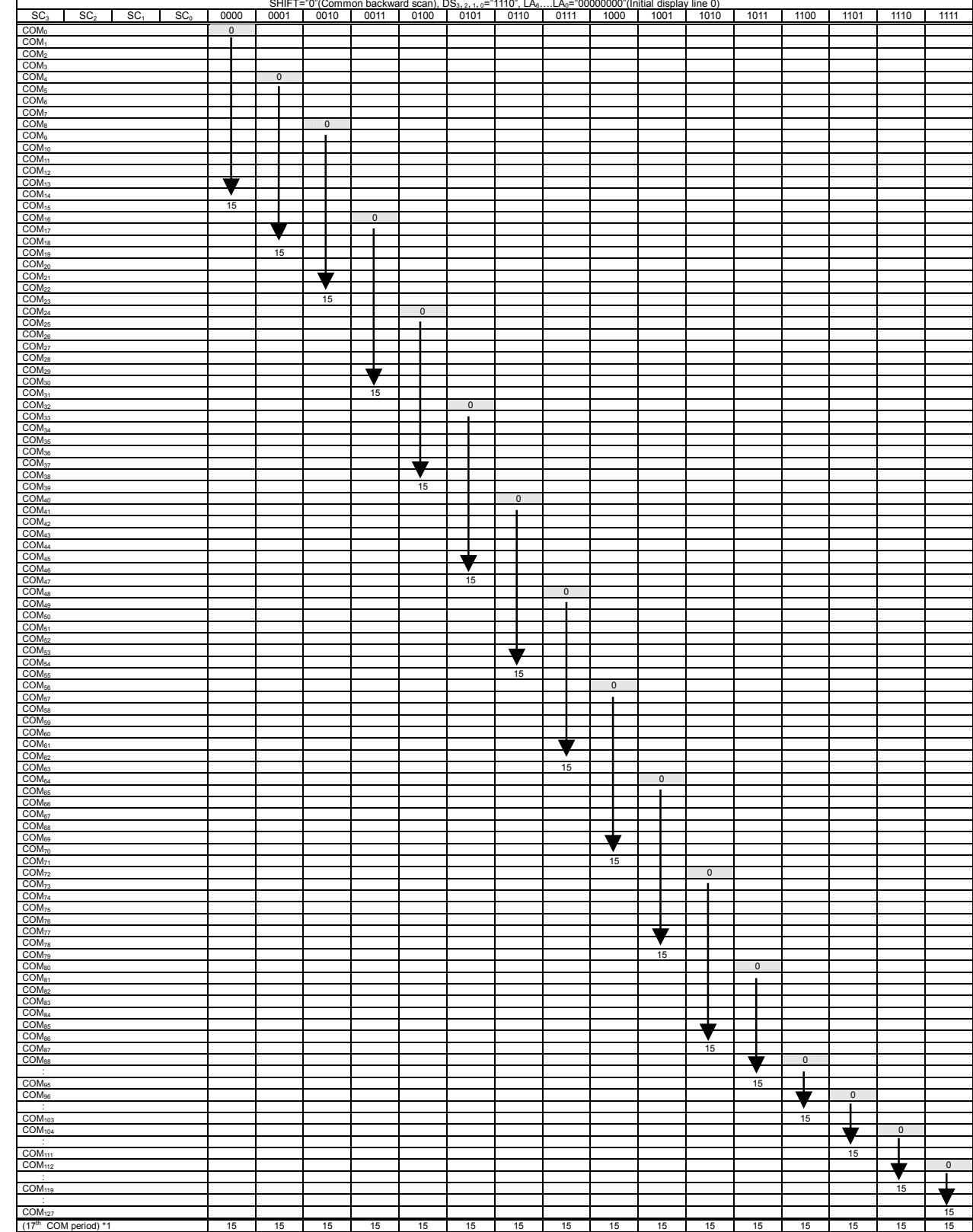
(33-2) Initial display line “0”, 1/17 duty cycle (Common backward scan, DSE=“0”)
