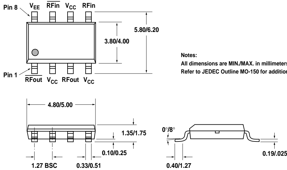
Figure 9. HMMC-3122 Package and Dimensions. (Available in near future.)
