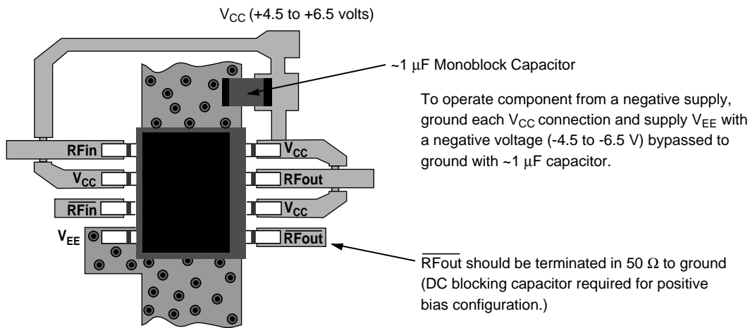
Figure 10. HMMC-3122 Assembly Diagram. (Single-supply, positive-bias configuration shown)
