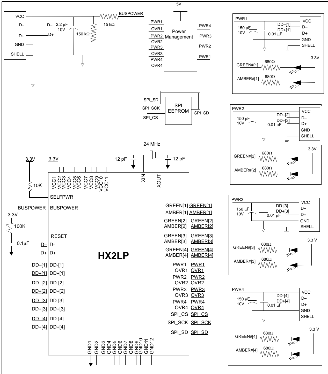
Figure 5. Sample Schematic
