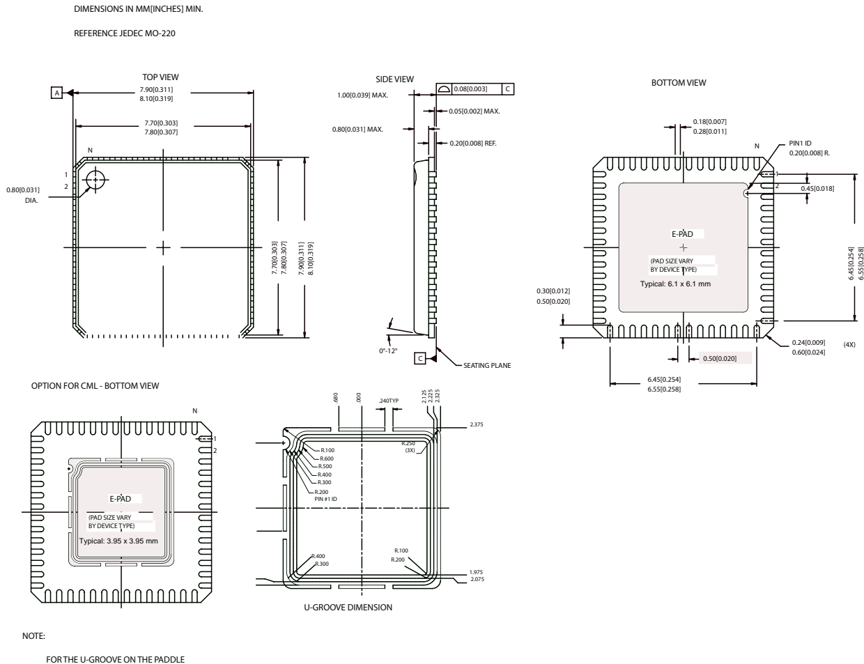
Figure 6. 56-Lead QFN 8 × 8 MM LF56A.
