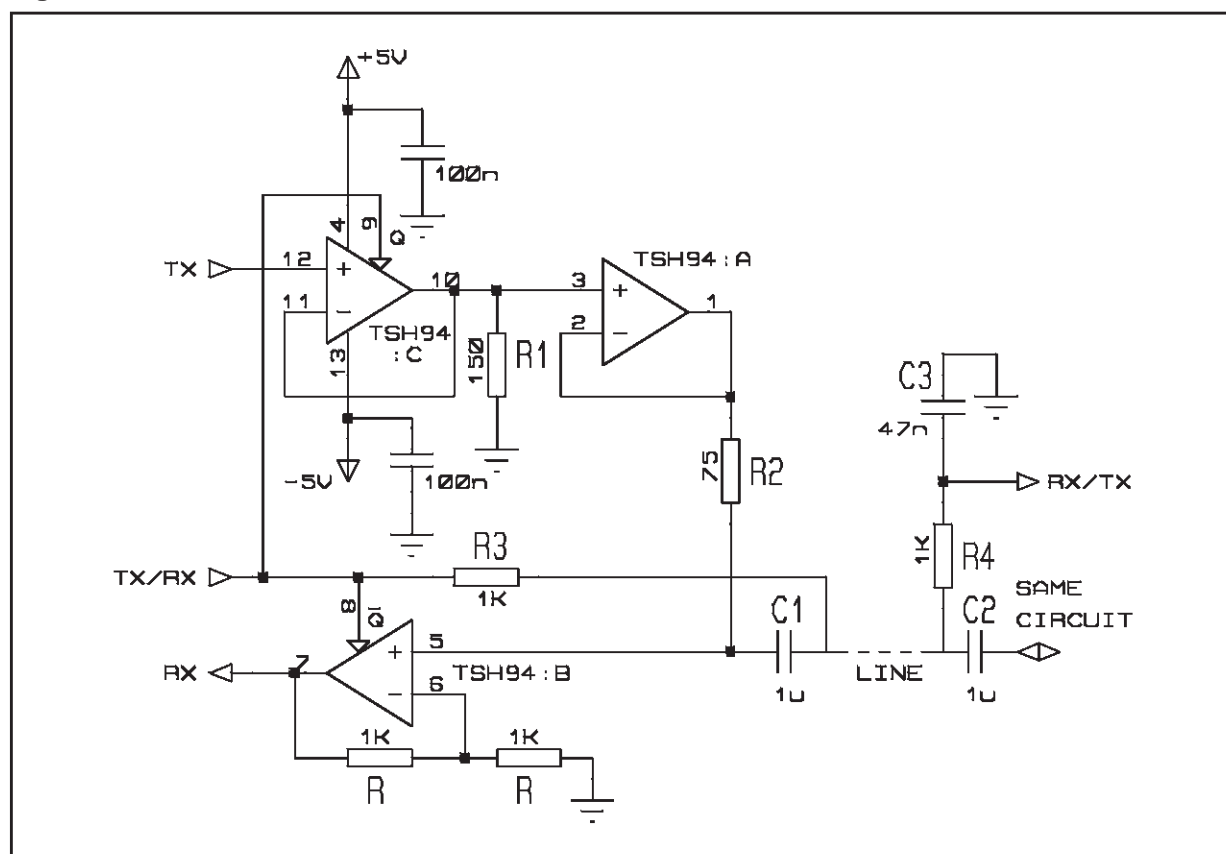
Figure 1 : Electrical Schematic
