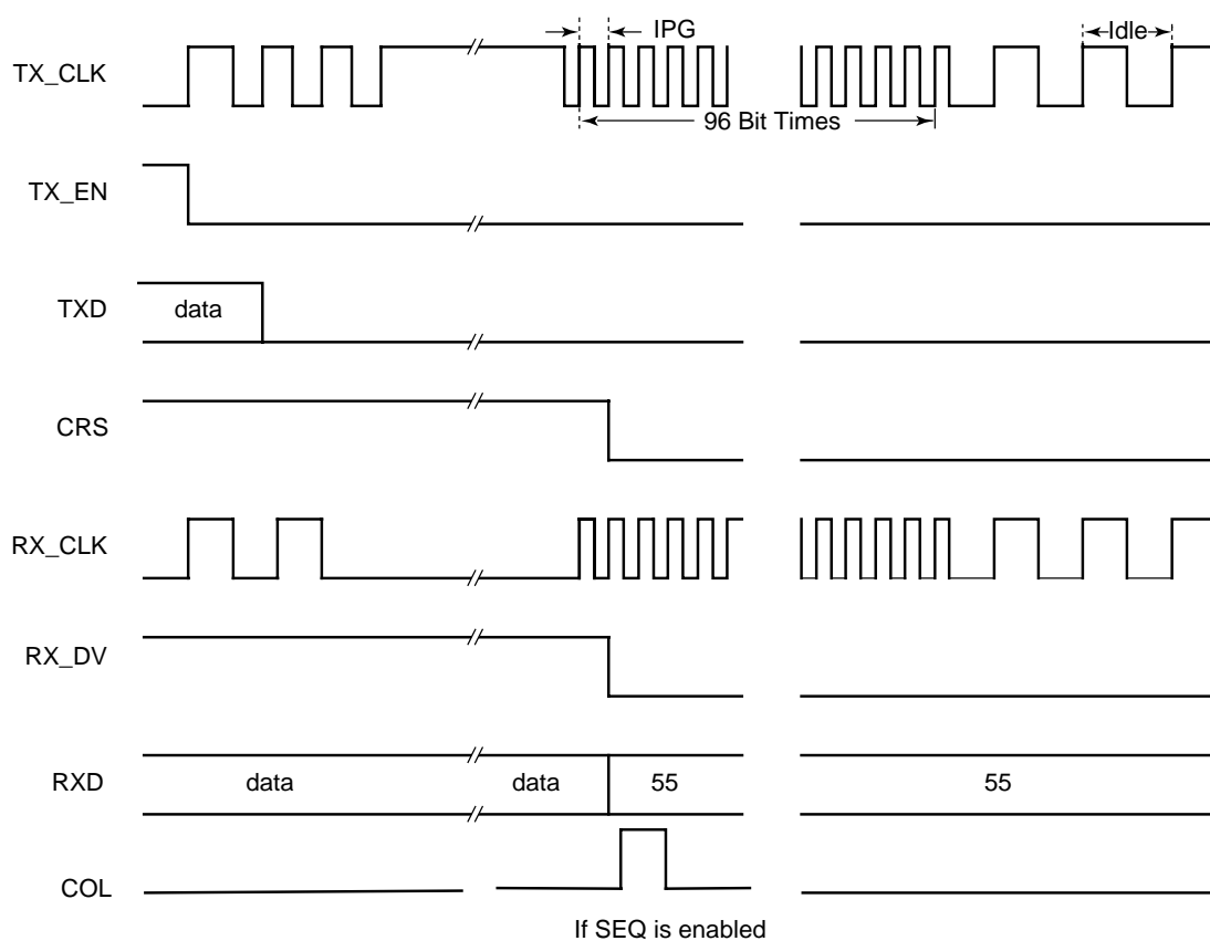
Figure 15. MII End of Transmission
