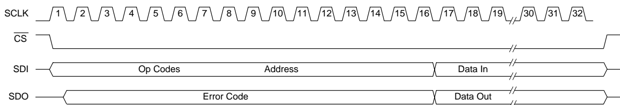
Figure 9. Operation of the SPI Interface
