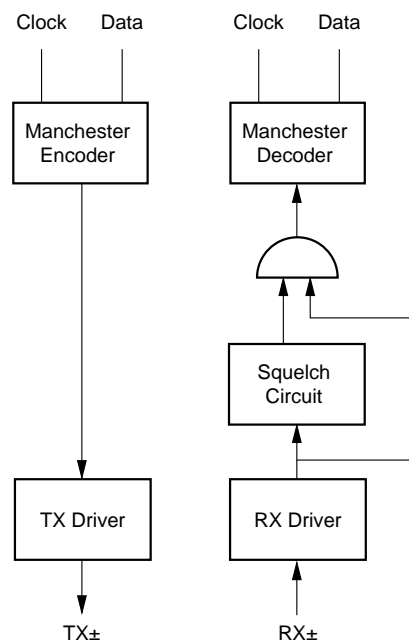
Figure 22. 10BASE-T Transmit and Receive Data Paths
