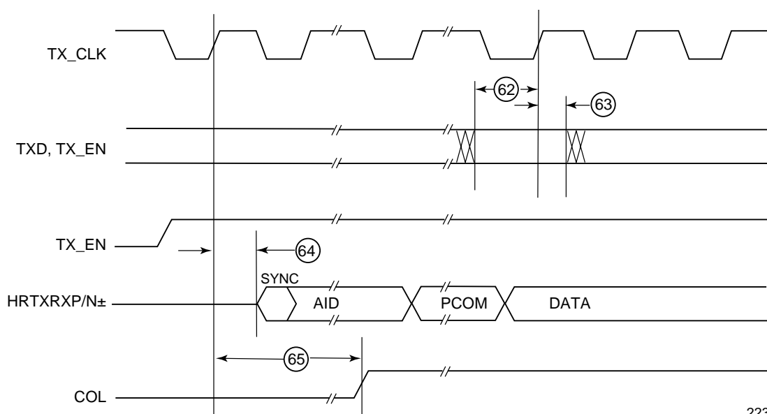
Figure 13. 1 Mbps HomePNA Transmit Timing (MII)
