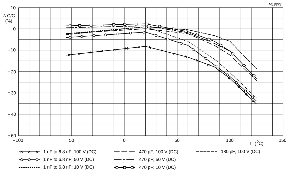
Fig.8 Typical capacitance change with respect to the capacitance value at 0 V and 20 °C as a function of temperature at different DC voltages.
