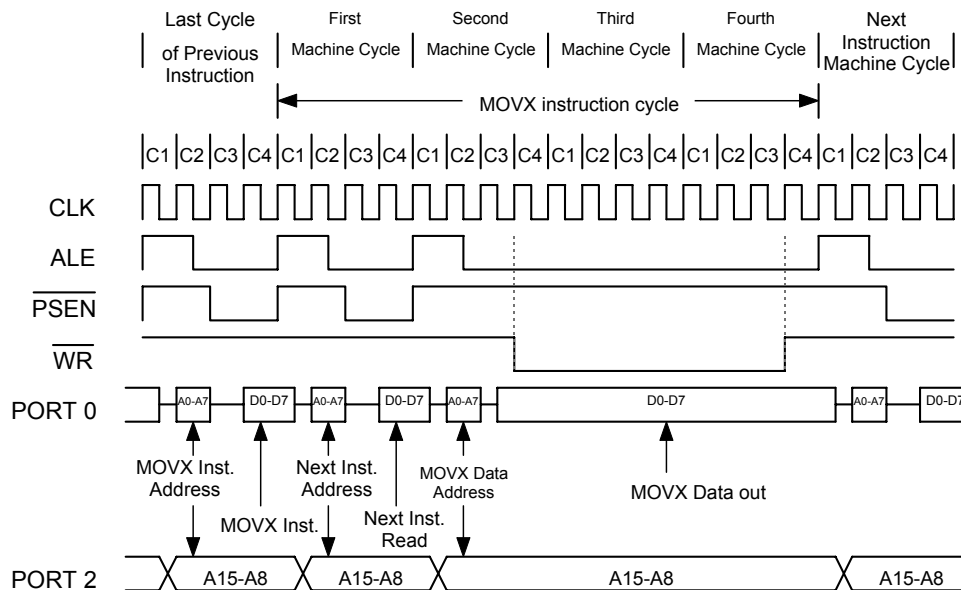
Figure 10. Data Memory Write with Stretch Value = 2
