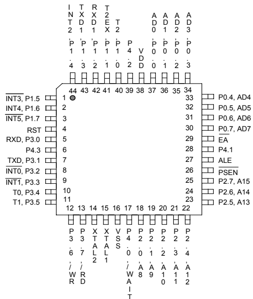
44-Pin QFP
