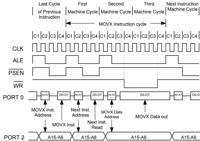
Figure 9. Data Memory Write with Stretch Value = 1
