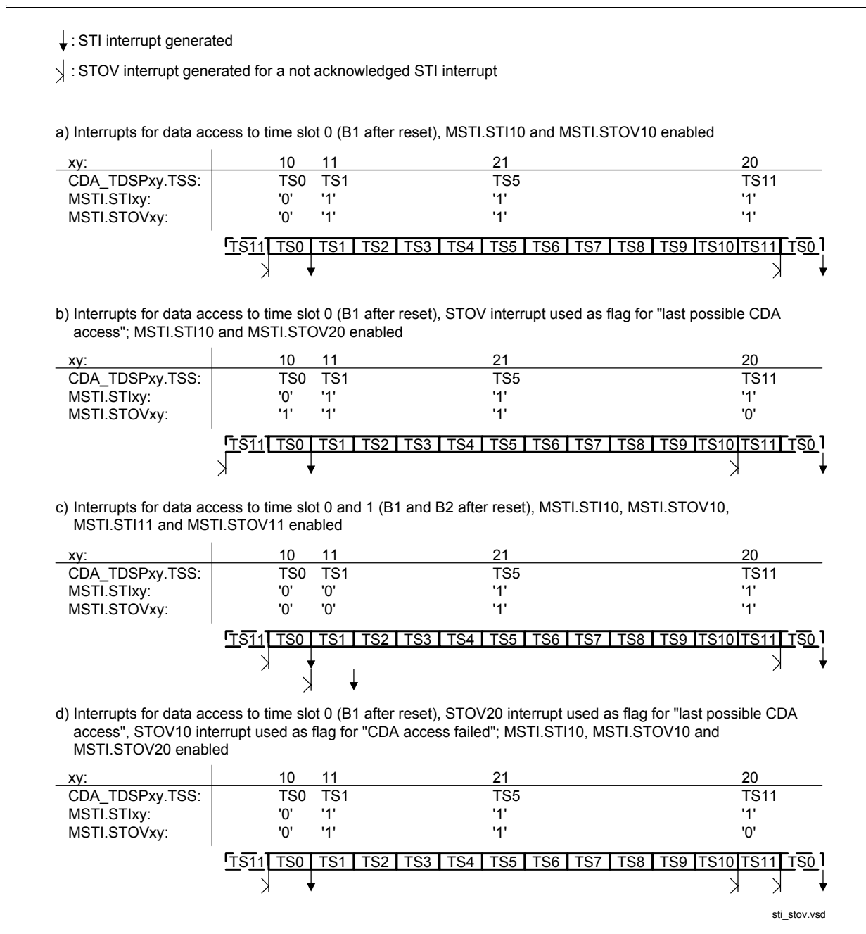
Figure 125 Examples for the Synchronous Transfer Interrupt Control with one enabled STIxy
