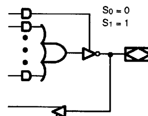
Combinatorial/Active Low
