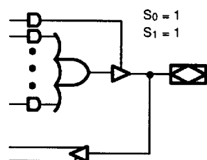
Combinatorial/Active High
