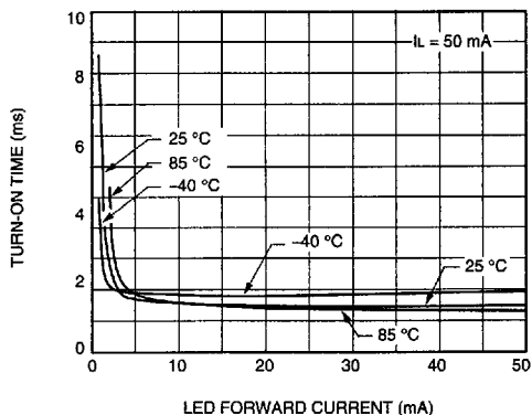
C. Turn-On Time vs. LED Current (LH1524)
