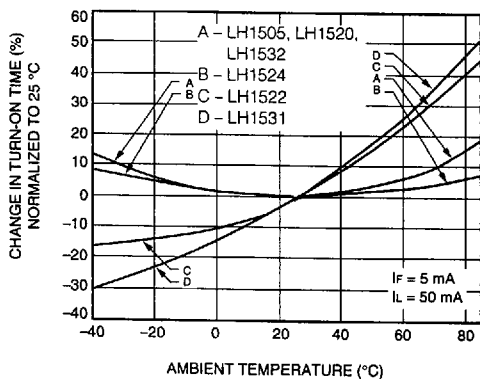
C. Turn-On Time vs. Temperature
