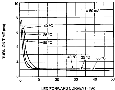
B. Turn-On Time vs. LED Current (LH1522)
