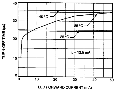
C. Turn-Off Time vs. LED Current (LH1544)
