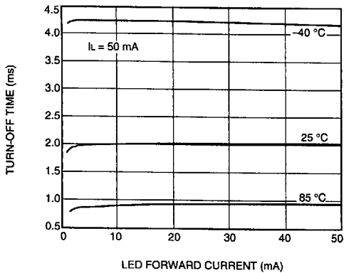
A. Turn-Off Time vs. LED Current (LH1524)
