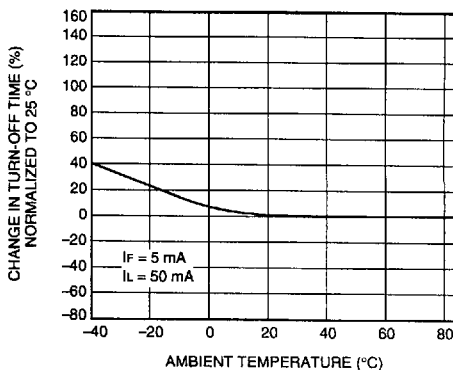
F. Turn-Off Time vs. Temperature (LH1544)
