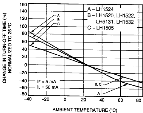
E. Turn-Off Time vs. Temperature
