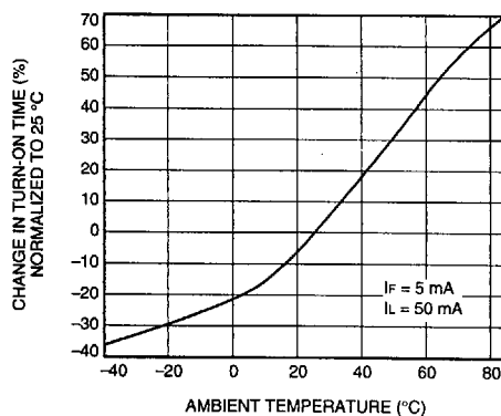
D. Turn-On Time vs. Temperature (LH1544)
