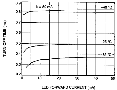
B. Turn-Off Time vs. LED Current (LH1531)
