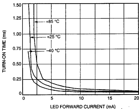
E. Turn-On Time vs. LED Current (LH1544)
