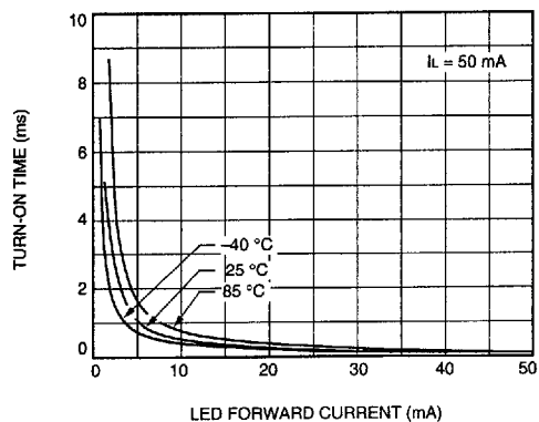
D. Turn-On Time vs. LED Current
