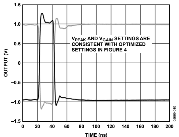
Figure 9. Equalized Pulse Response for 50 M of Cable
