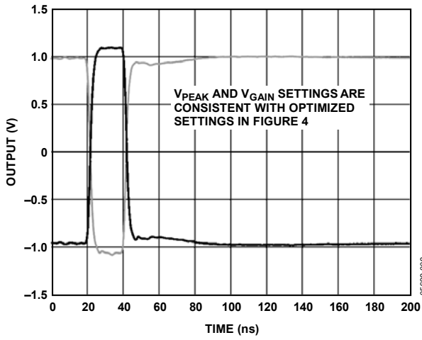
Figure 10. Equalized Pulse Response for 100 M of Cable
