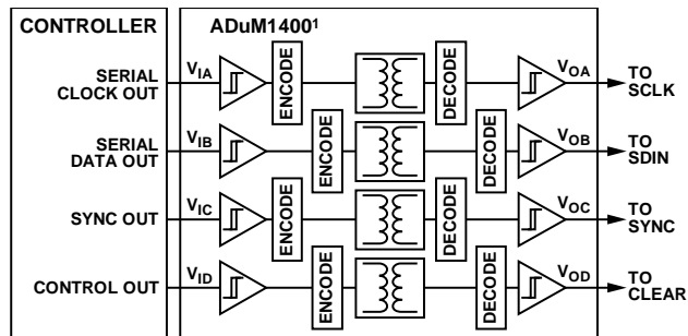
Figure 56. Isolated Interface
