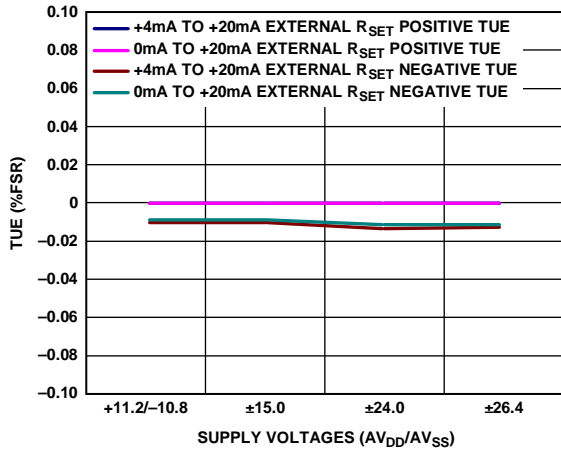
Figure 30. Total Unadjusted Error Current Mode, External R_{SET} Sense Resistor
