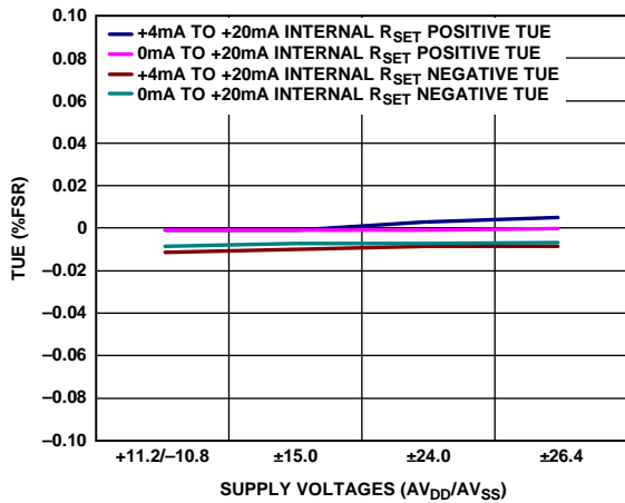
Figure 31. Total Unadjusted Error Current Mode, Internal R_{SET} Sense Resistor
