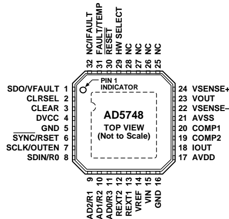
Figure 4. Pin Configuration
