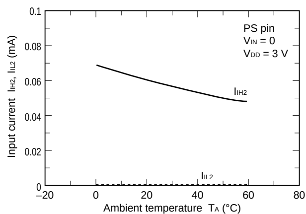
I_{IH2} vs. T_A Characteristics
