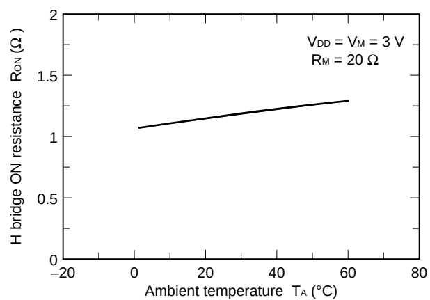
R ON vs. T A Characteristics
