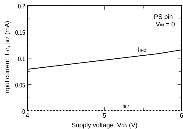
I_{IH2} vs. V_{DD} Characteristics
