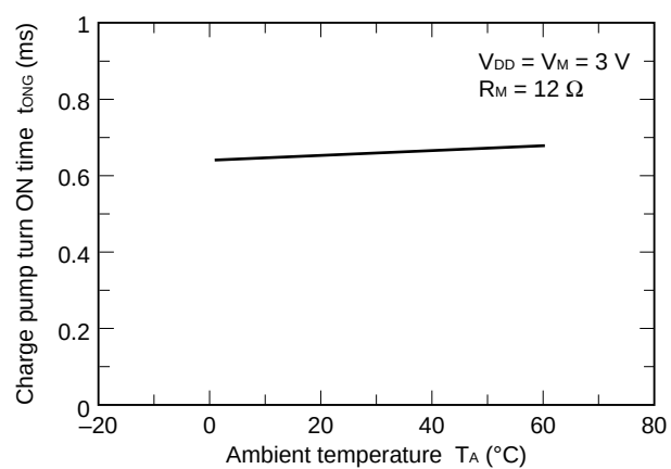
t ON vs. T A Characteristics
