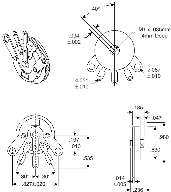
Dimensions (In.)
