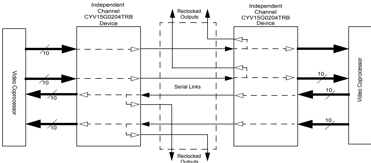
Figure 1. HOTLink II™ System Connections
