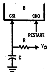
RC Oscillator
