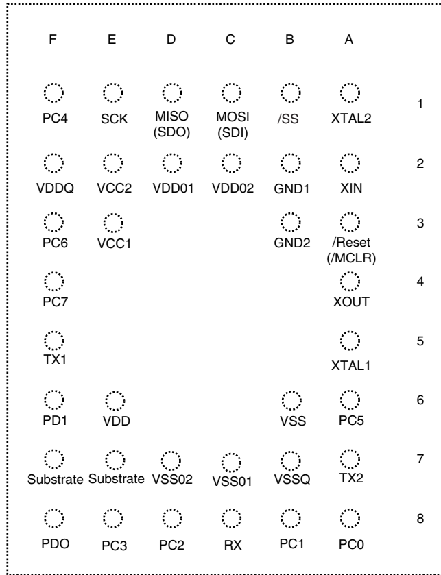
Figure 3. LBGA36 Package Pinout
