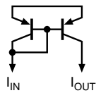
Figure 2. Simple PNP Current Source. Has Slower Frequency Response, and up to ±15% Tolerance Error. I_{OUT} = I_{IN} * (1 + 2/\beta)
