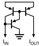
Figure 3. Widlar Current Source, Moderate Frequency Response. I_{OUT} = I_{IN} * (1 + 2/\beta^2)
