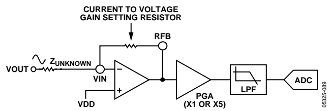
Figure 20. AD5934 System Voltage Gain
