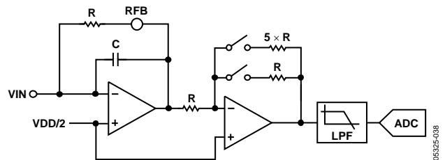
Figure 17. AD5934 Receive Stage
