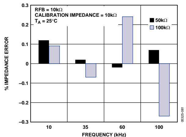
Figure 24. Range 3: Typical % Impedance Error over Frequency
