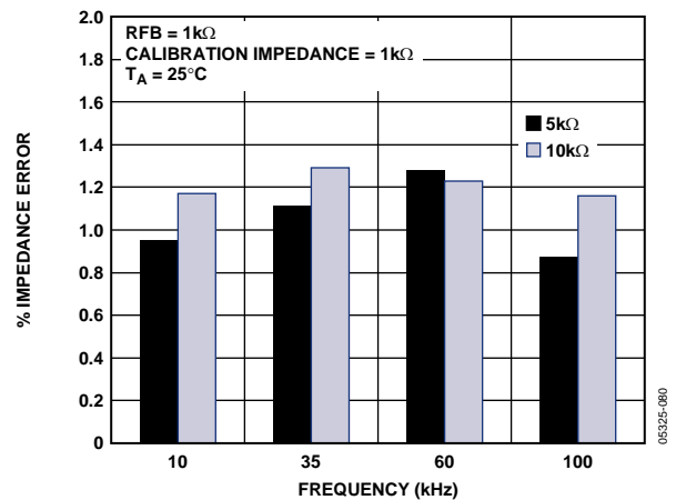
Figure 23. Range 2: Typical % Impedance Error over Frequency
