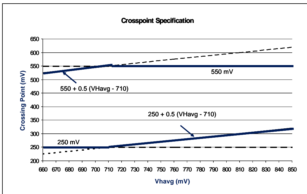
Figure 10. Differential Clock Crosspoint Specification
