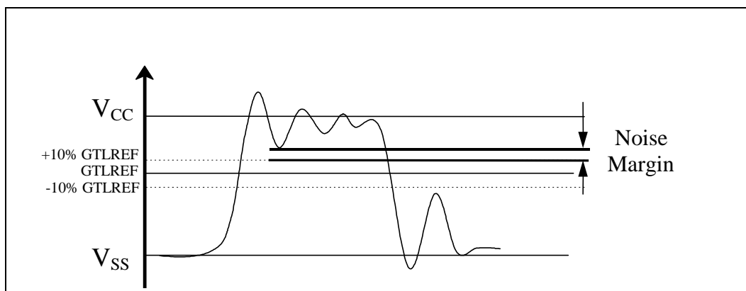
Figure 24. Low-to-High System Bus Receiver Ringback Tolerance
