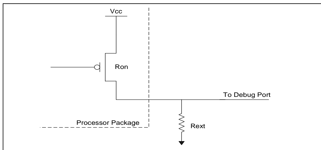
Figure 6. ITPCLKOUT[1:0] Output Buffer Diagram
