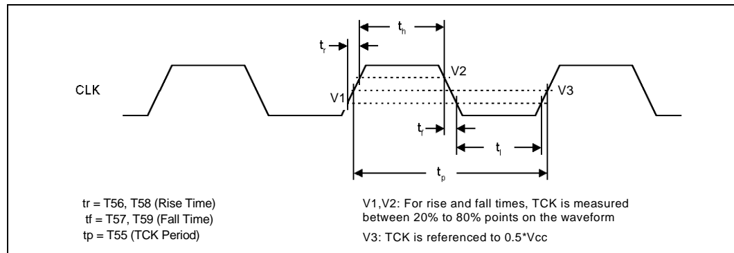
Figure 8. TCK Clock Waveform
