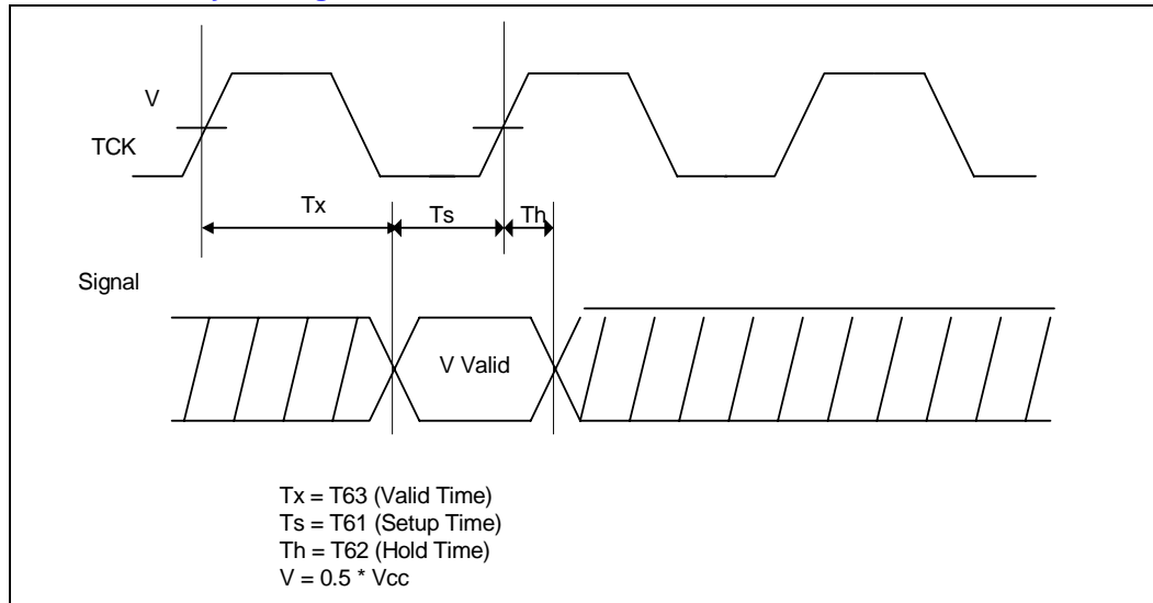
Figure 20. TAP Valid Delay Timing
