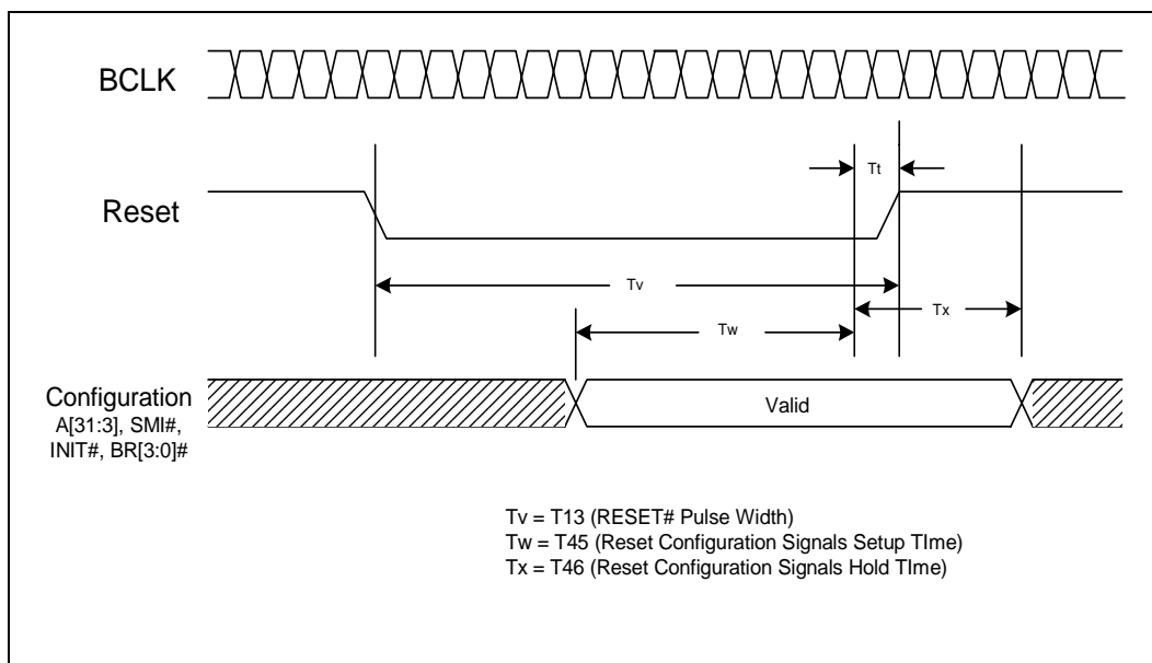
Figure 12. System Bus Reset and Configuration Timings
