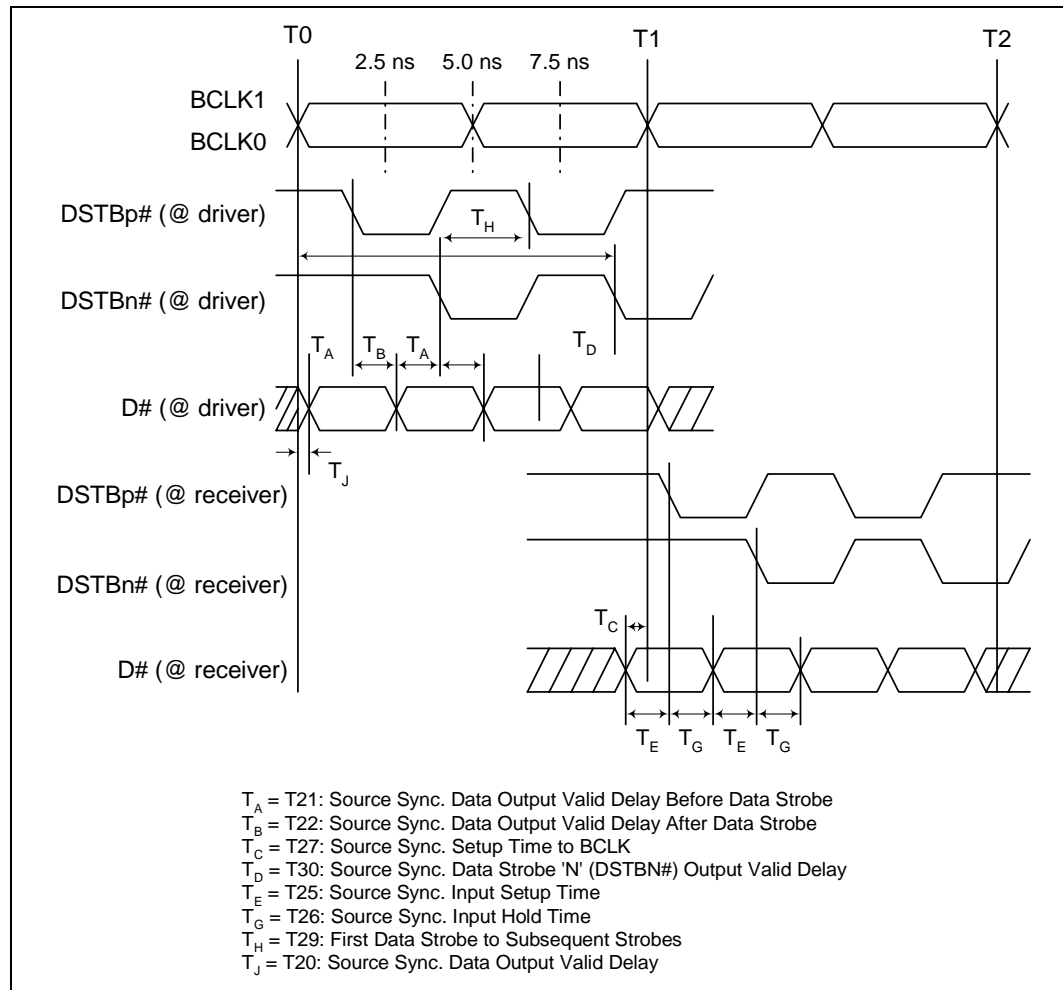
Figure 14. Source Synchronous 4X Timings
