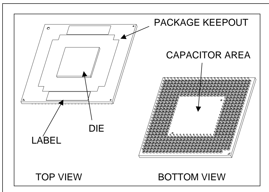
Figure 29. Micro-FCPGA Package Top and Bottom Isometric Views
