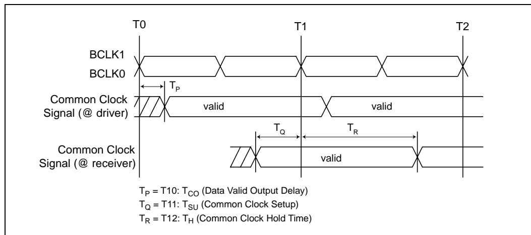
Figure 11. System Bus Common Clock Valid Delay Timings
