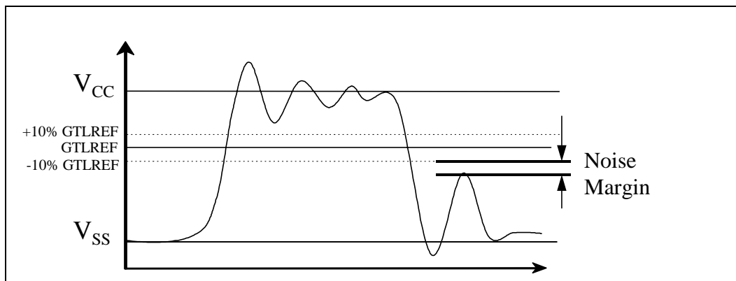
Figure 25. High-to-Low System Bus Receiver Ringback Tolerance
