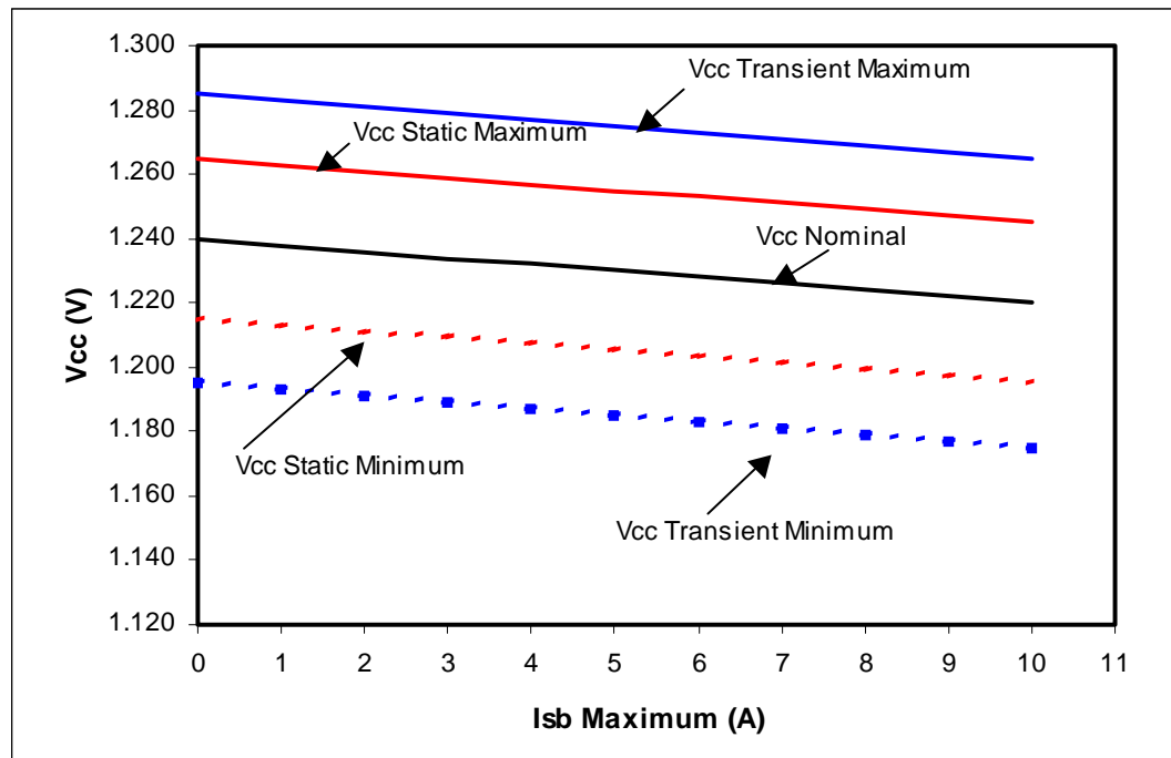
Figure 5. Illustration of Deep Sleep V_{CC} Static and Transient Tolerances (VID Setting = 1.30 V)
