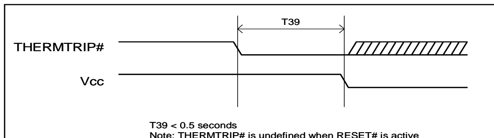
Figure 18. THERMTRIP# to Vcc Timing
