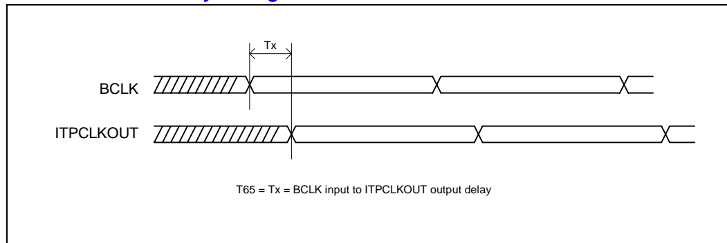
Figure 21. ITPCLKOUT Valid Delay Timing
