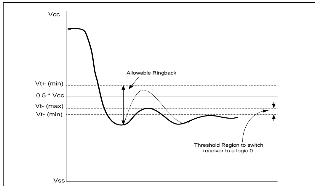
Figure 27. High-to-Low System Bus Receiver Ringback Tolerance for PWRGOOD and TAP Buffers
