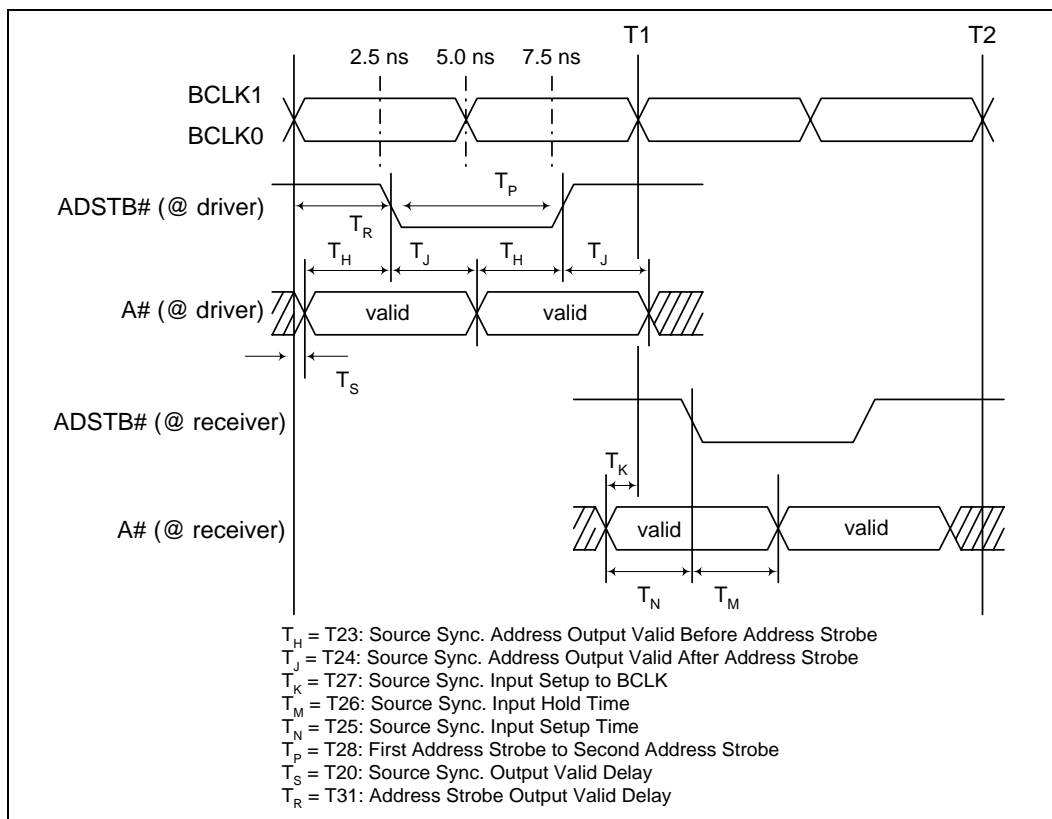
Figure 13. Source Synchronous 2X (Address) Timings
