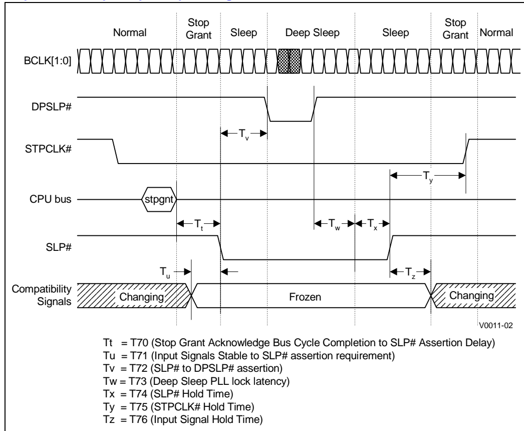
Figure 22. Stop Grant/Sleep/Deep Sleep Timing
