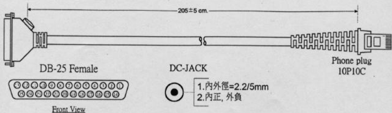
NEW CCD (1067, 1090)R CABLE with DB-25F and DC-JACK(standard pin assignment)
