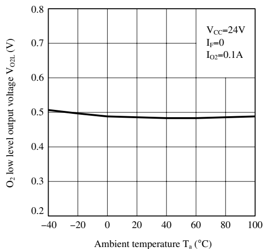
Fig.21 O 2 Low Level Output Voltage vs. Ambient Temperature
