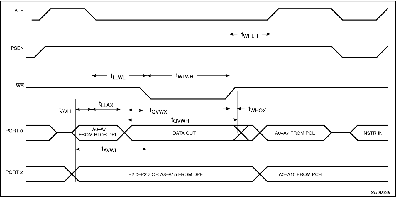
Figure 30. External Data Memory Write Cycle
