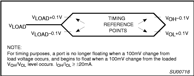
Figure 34. Float Waveform
