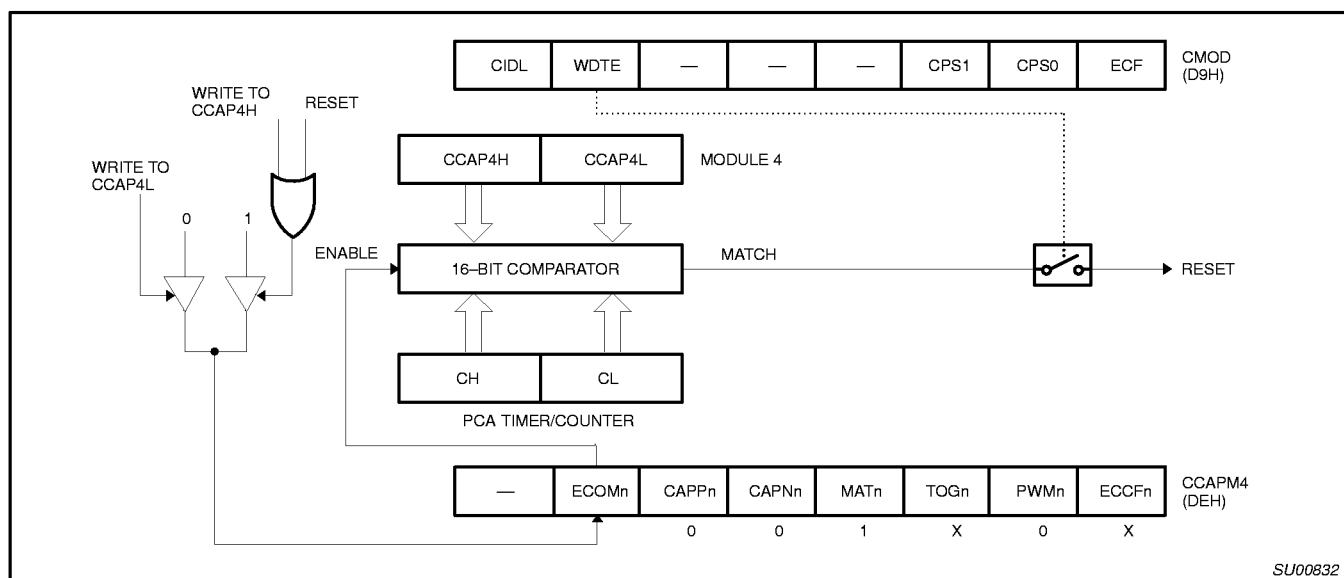
Figure 24. PCA Watchdog Timer m(Module 4 only)
