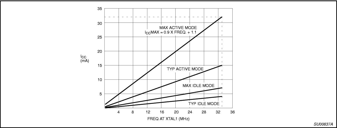
Figure 35. I_{CC} vs. FREQ Valid only within frequency specifications of the device under test
