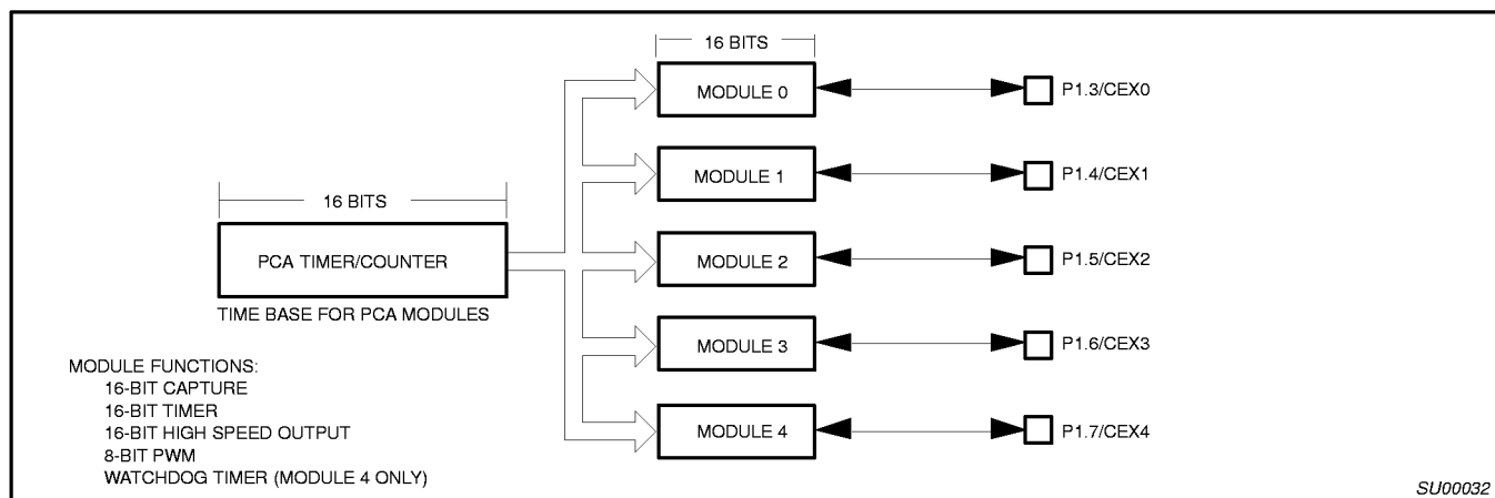
Figure 13. Programmable Counter Array (PCA)
