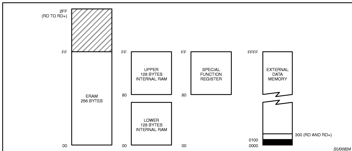
Figure 27. Internal and External Data Memory Address Space with EXTRAM = 0
