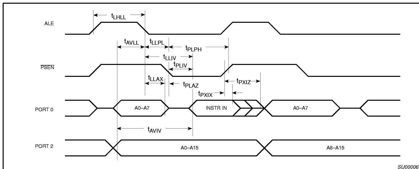
Figure 28. External Program Memory Read Cycle
