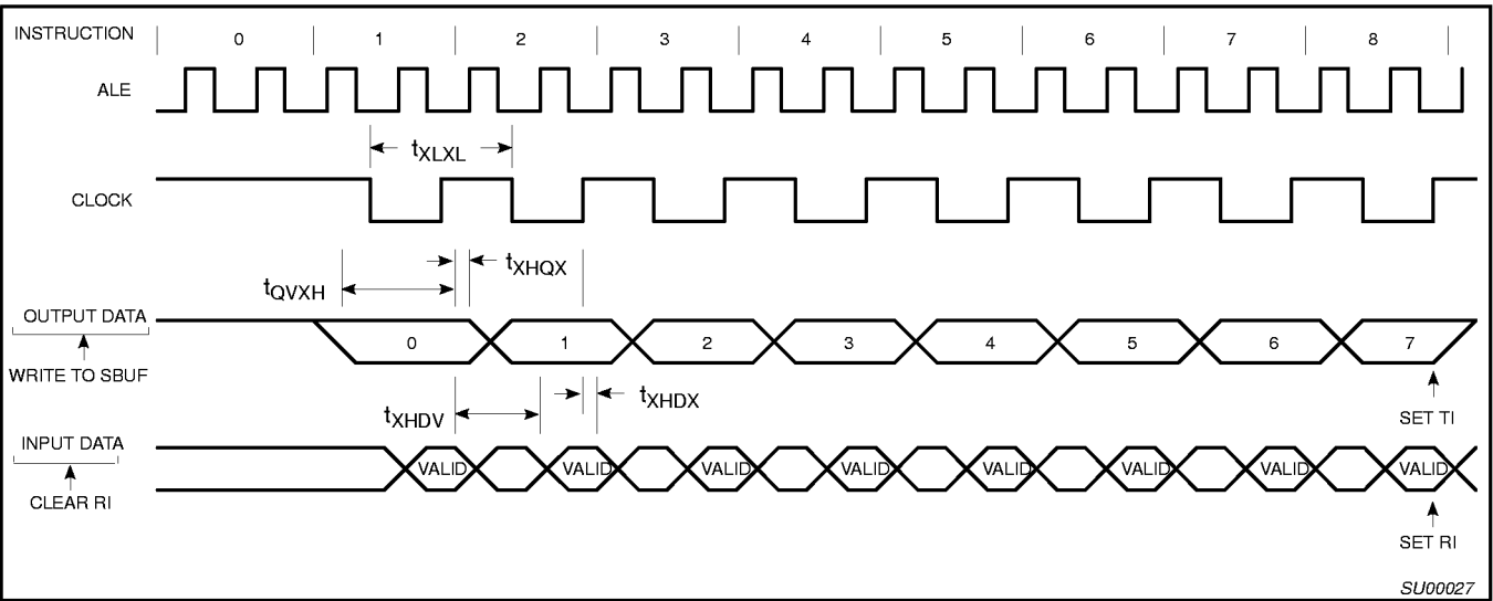
Figure 31. Shift Register Mode Timing
