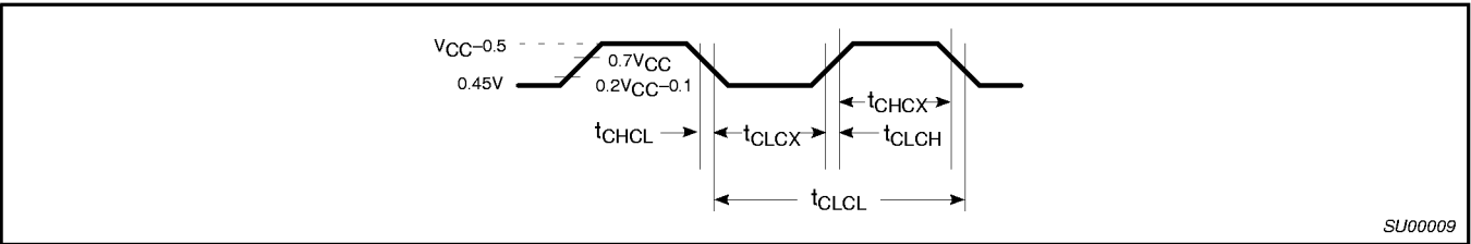
Figure 32. External Clock Drive
