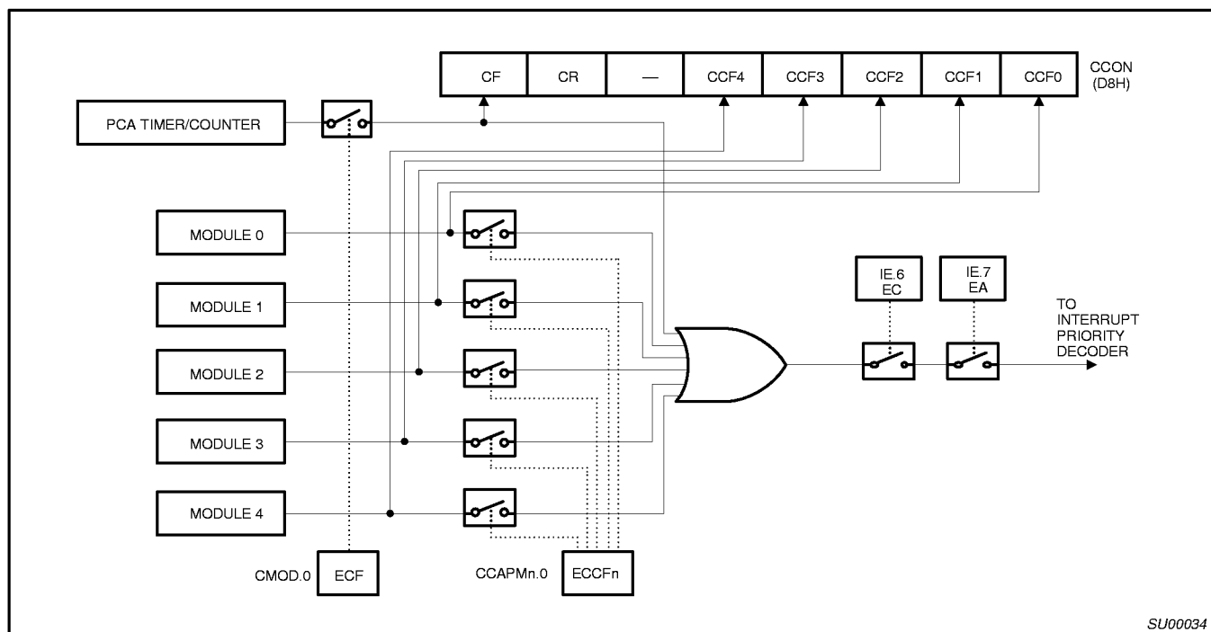
Figure 15. PCA Interrupt System
