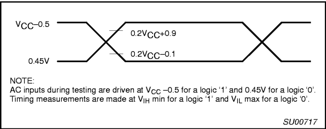
Figure 33. AC Testing Input/Output
