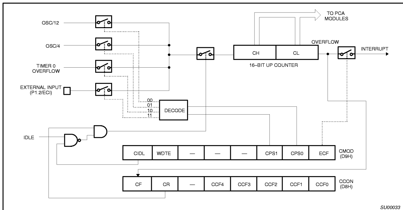
Figure 14. PCA Timer/Counter
