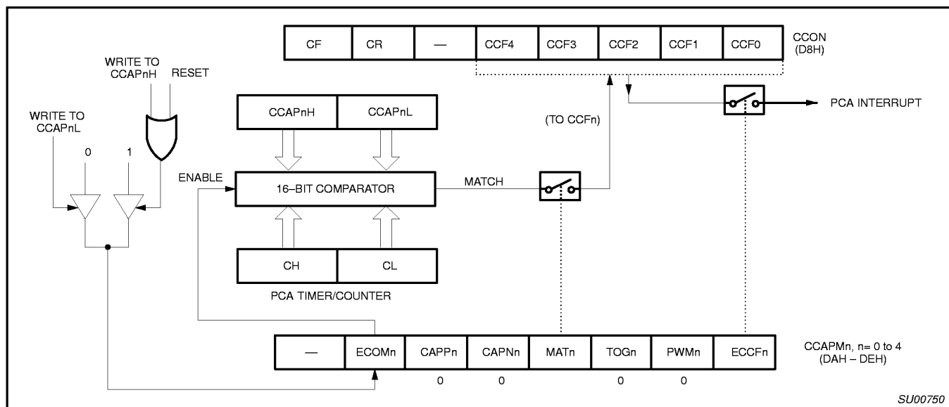
Figure 21. PCA Compare Mode
