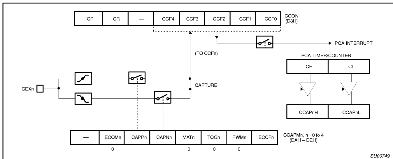
Figure 20. PCA Capture Mode
