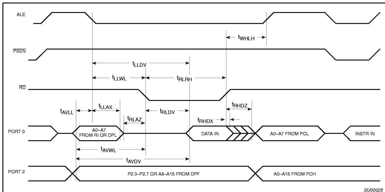
Figure 29. External Data Memory Read Cycle
