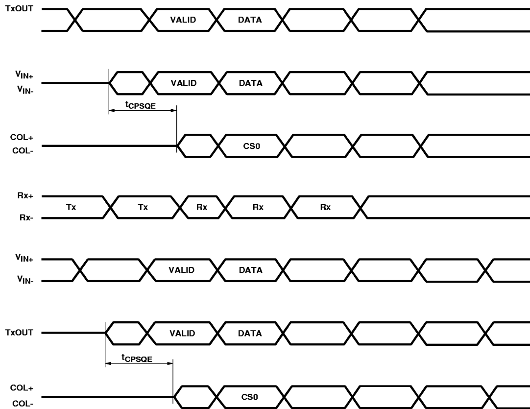
Figure 8. Collision Timing.
