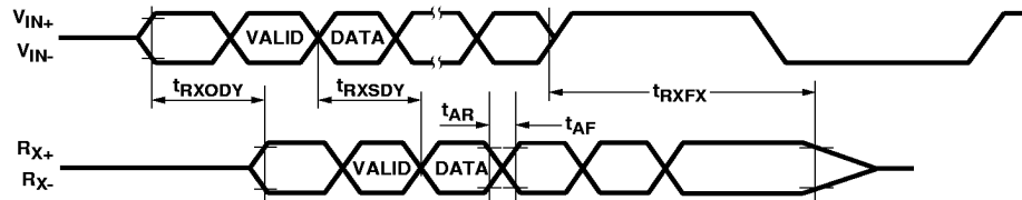
Figure 7. Receive Timing.
