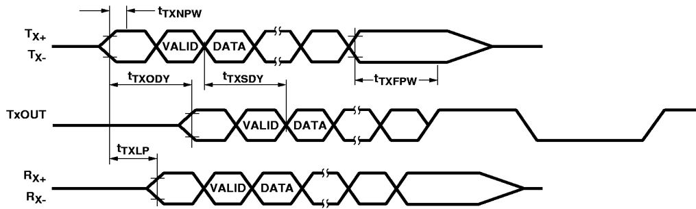
Figure 6. Transmit and Loopback Timing.
