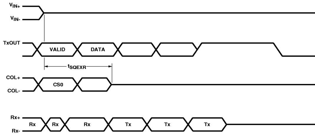
Figure 9. Collision Timing.
