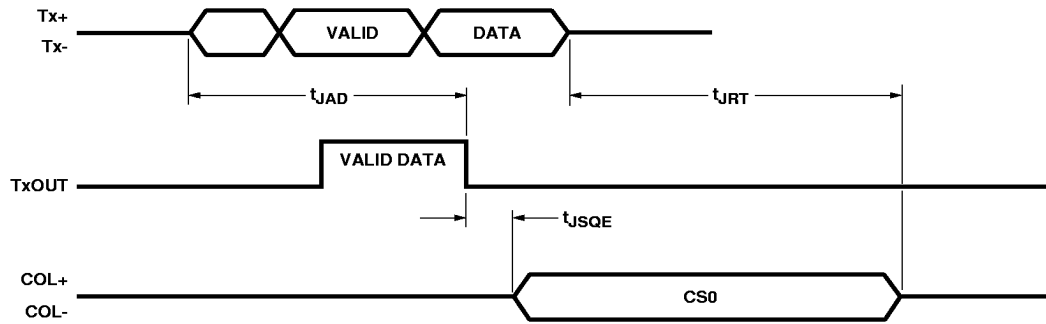
Figure 12. Jabber Timing.
