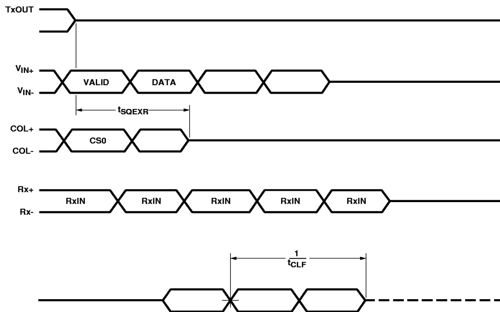
Figure 10. Collision Timing.
