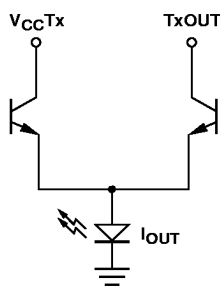
Figure 2. Fiber Optic LED Driver Structure.
