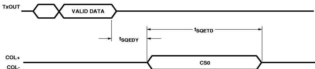
Figure 11. SQE Timing.
