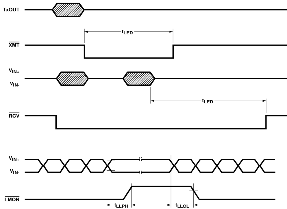
Figure 13. LED Timing.
