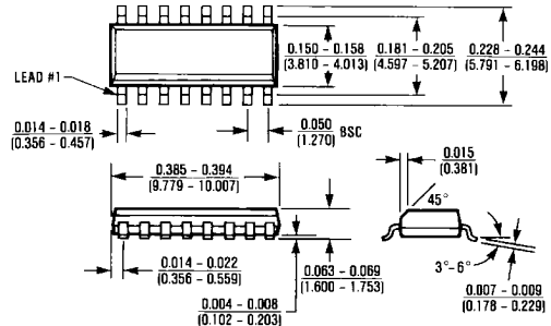
16 Lead Small Outline (SE)
