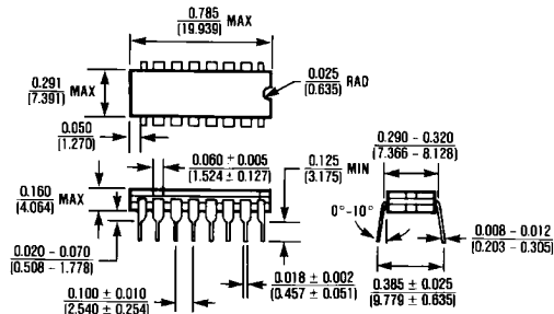
16 Lead Cerdip
