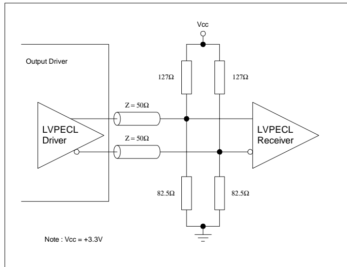
Figure 3 - LVPECL Output Termination Circuit
