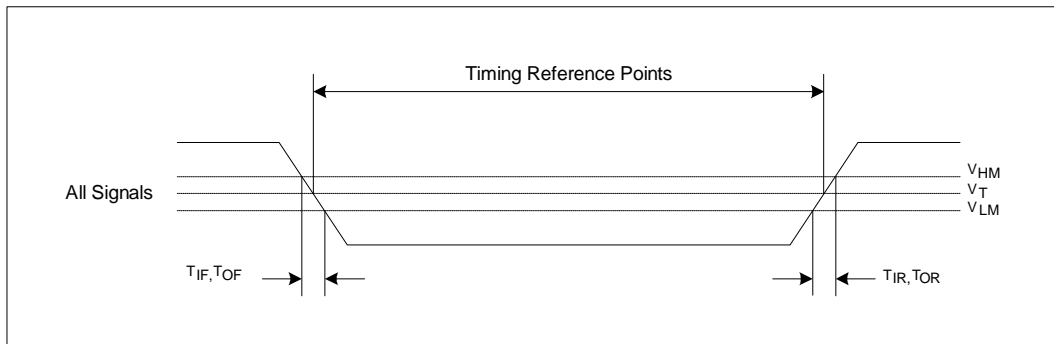
Figure 11 - Timing Parameters Measurement Voltage Levels
