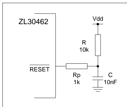
Figure 5 - Simple Reset Circuit
