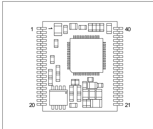
Figure 2 - 40 Pin SMT DIL Top View
