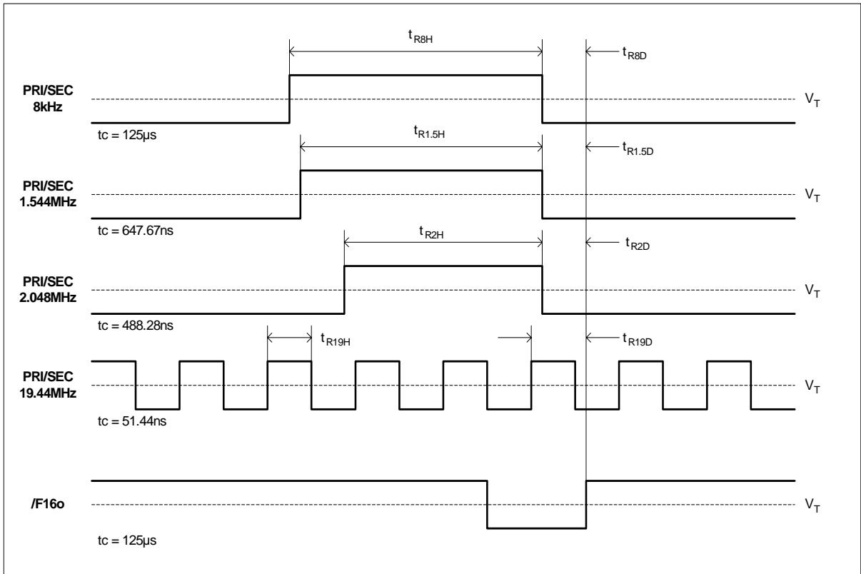
Figure 12 - Input to Output Timing (Normal Mode)
