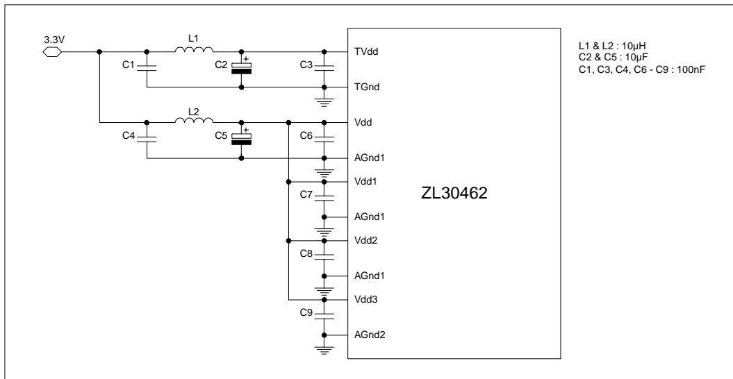
Figure 10 - Power Supply Decoupling
