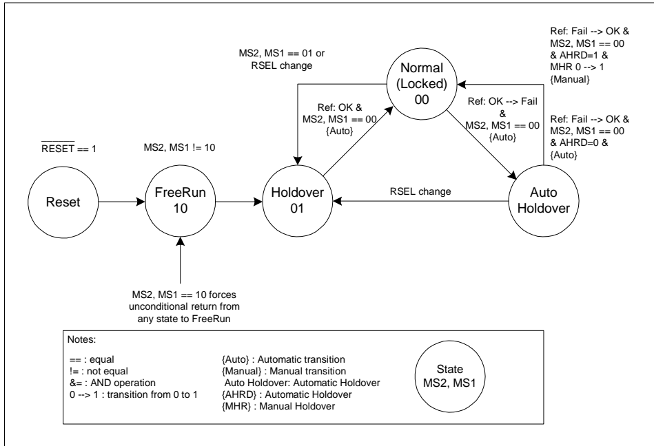
Figure 4 - ZL30462 State Machine
