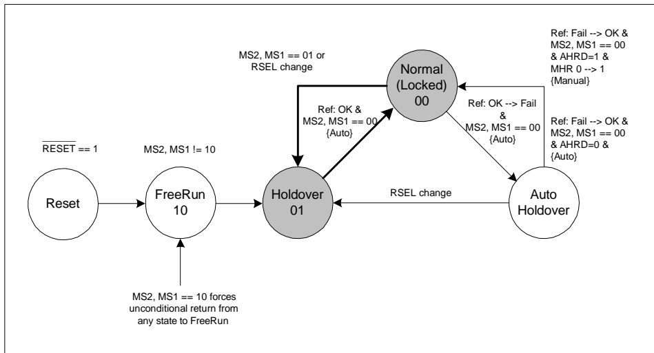
Figure 9 - Manual Reference Switching
