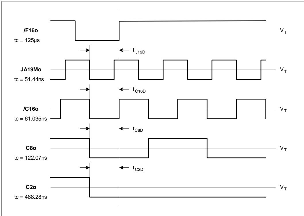
Figure 14 - Output Timing
