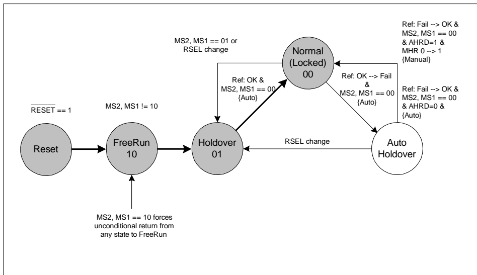
Figure 6 - Transition from Free-run to Normal mode
