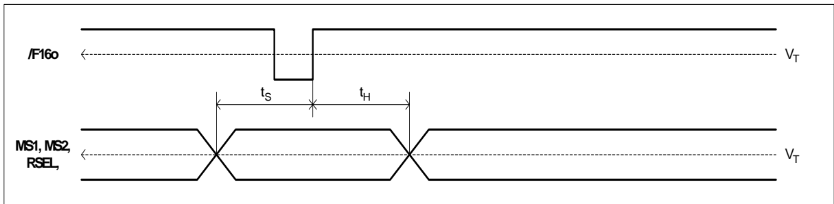
Figure 13 - Input Control Signal Setup and Hold Time
