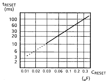
C_{RESET} - t_{RESET} TYPICAL CURVE
