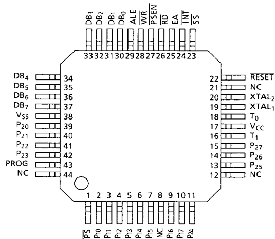
Figure 2.1 Micro Flat Package Pin Connections
