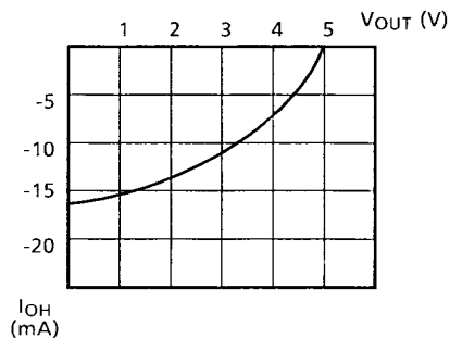
V_{OUT} - I_{OH} TYPICAL CURVE (DB, CONTROL)
