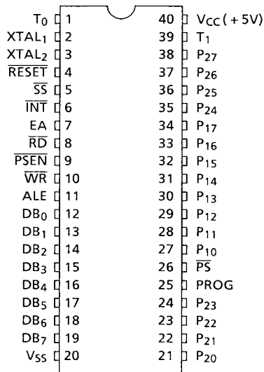
Figure 2.1 DIP Pin Connections
