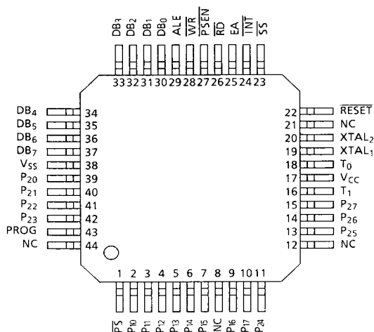
Figure 2.1 (2) Micro Flat Package Pin Connections
