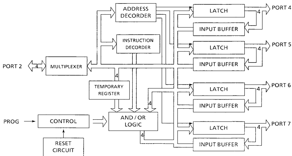
Figure 2.2 Block Diagram
