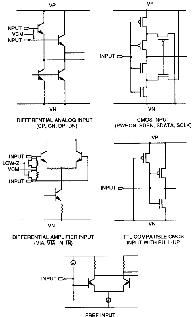
FIGURE 17: Input Structures
