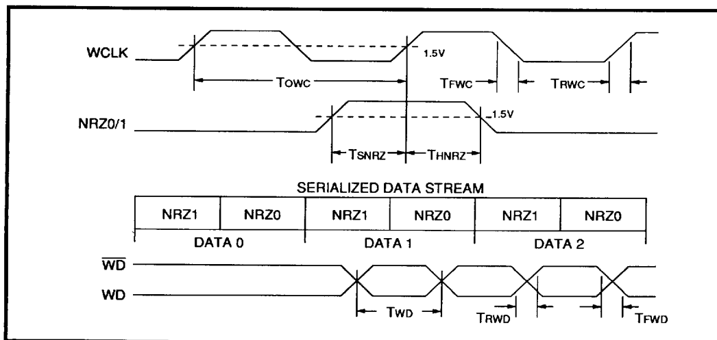
FIGURE 20: \overline{\text{WD}} and NRZ Write Timing
