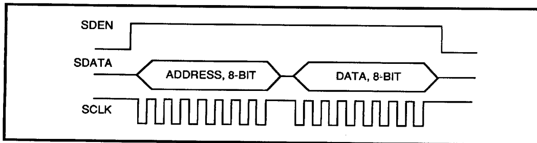
FIGURE 16: Serial Port Transfer Format
