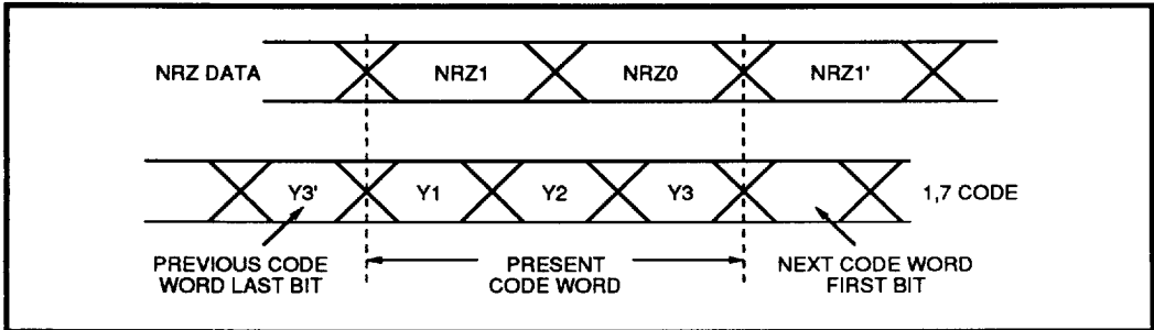
FIGURE 15: NRZ Data Word to 1,7 Code Word Bit Comparison (Reference Table 7 for decode scheme)
