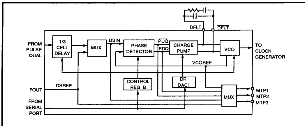
FIGURE 11: Data Separator Phase Locked Loop
