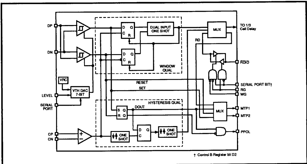
FIGURE 3: Pulse Qualification
