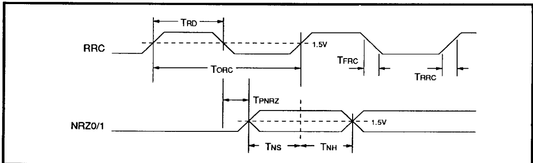
FIGURE 19: NRZ Read Timing
