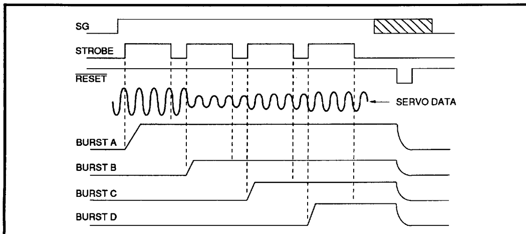
FIGURE 7: Servo Capture Timing Diagram
