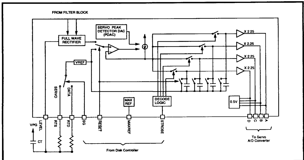
FIGURE 6: Servo Capture
