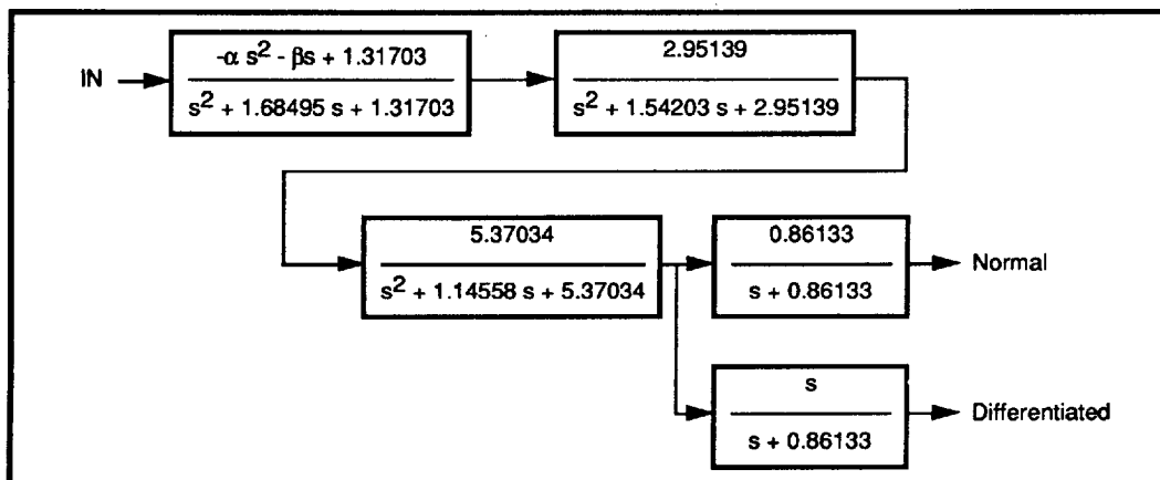
FIGURE 9: Normal Transfer Function Diagram
