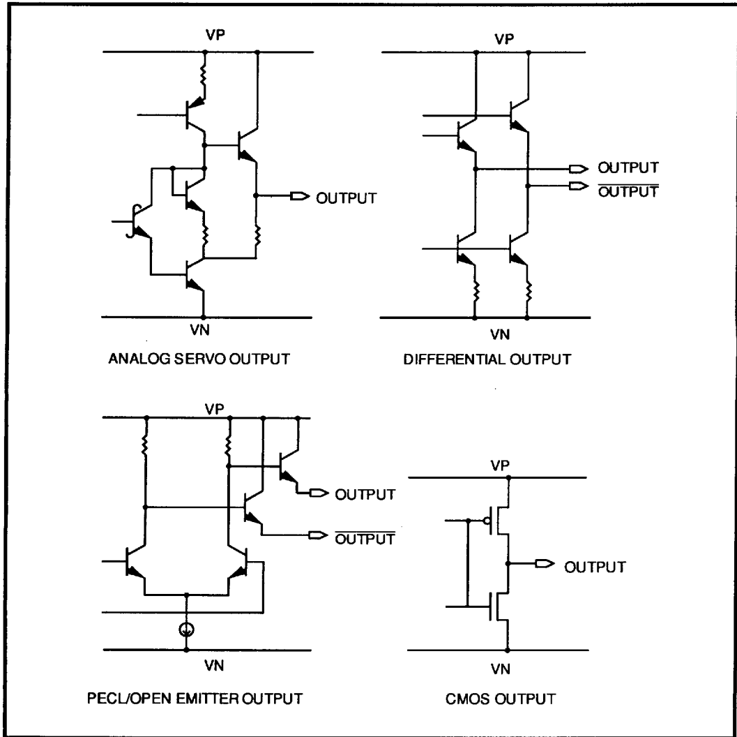
FIGURE 18: Output Structures
