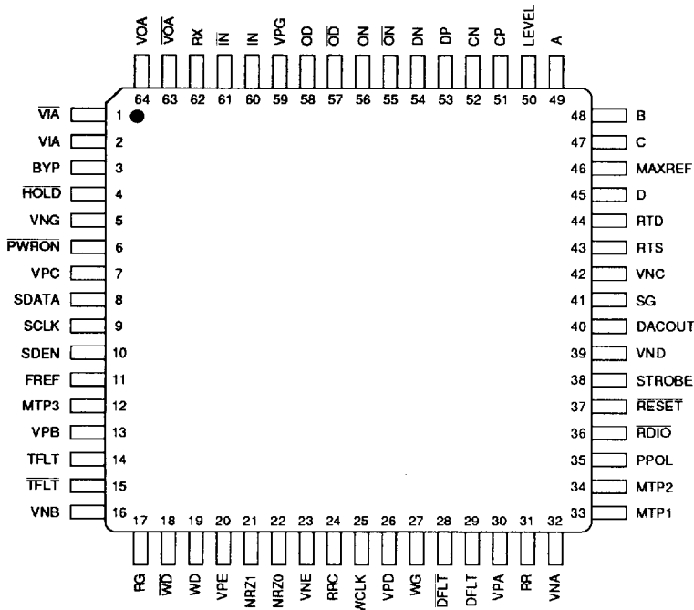
32P4752 64-Lead TQFP
