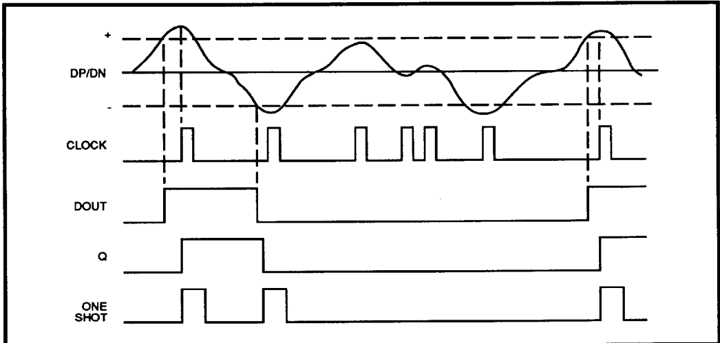
FIGURE 5: Hysteresis Comparator Timing Diagram
